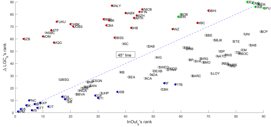
Figure 10: Comparison of the ranks of \text{InOut}_k and \Delta\text{LGC}_k : pre-crisis period
