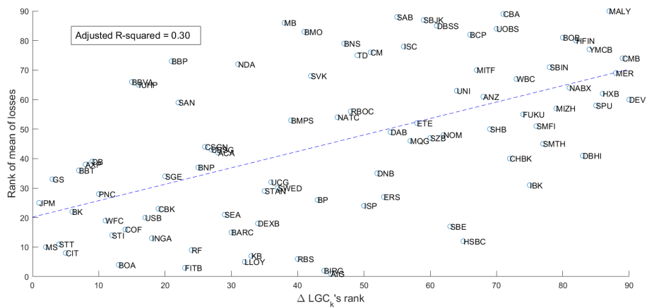
Figure B3: Systemic risk contributions \Delta LGC_k and mean of realized losses: \delta = -5\%
