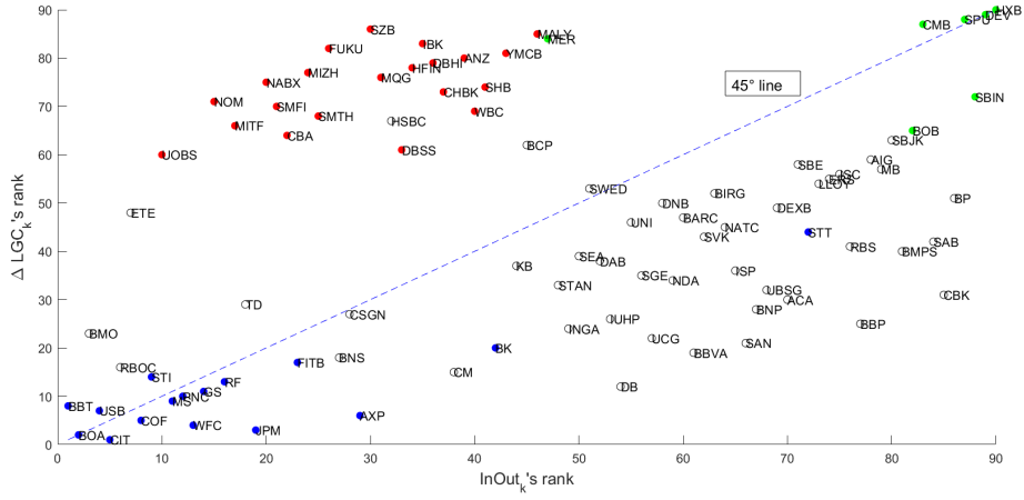
Figure 11: Comparison of the ranks of \text{InOut}_k and \Delta\text{LGC}_k : crisis period
