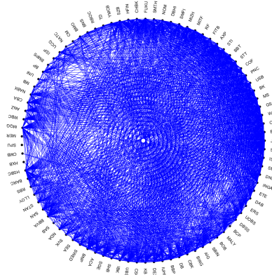
Figure B1: Network for the system excluding Ping An Bank: pre-crisis period
