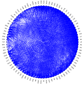
Figure 8: Network for all 90 banks: pre-crisis period
