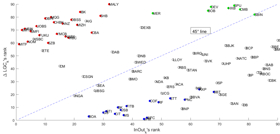
Figure B2: Comparison of the ranks of \text{InOut}_k and \Delta\text{LGC}_k : post-crisis period
