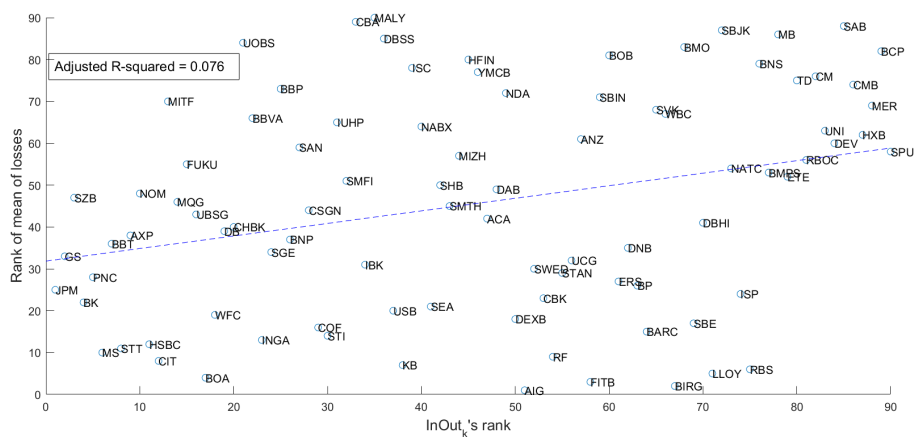
Figure B4: Systemic risk contributions \ln Out_k and mean of realized losses: \delta = -5\%
