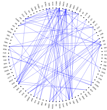
Figure 9: Network for the system excluding JPMorgan Chase & Co: pre-crisis period
