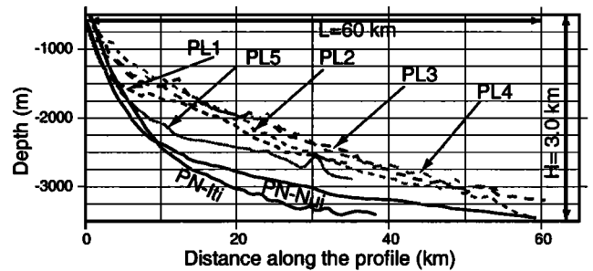
Figure 4. Bathymetric profiles across the landslide deposits (PL1 to PL4) and bathymetric profiles of Tahiti Nui and Tahiti Iiti in an area not covered by landslide deposits (PN-Nui and PN-Iiti).
