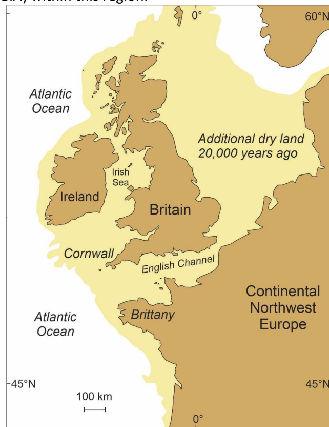
Figure 1. Northwest Europe showing the additional dry land that existed 20,000 years ago during the Last Glacial Maximum and which was progressively submerged in its aftermath (after Gaffney et al., 2009).
