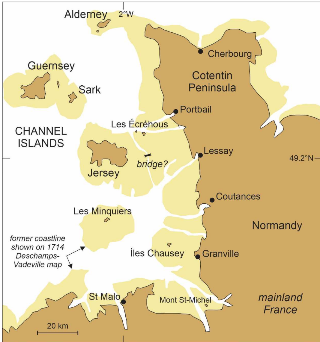
Figure 4. The Channel Islands and adjacent parts of France showing the former coastline as represented in the 1714 Deschamps-Vadville map (Chèvremont, 1882). It is possible that this map was copied from a Roman map that used oral memories to reconstruct an earlier coastline. Corroborative details may be preserved in traditions like that which recalled when Jersey residents might walk to (what is now) mainland France utilizing a bridge at one point.
