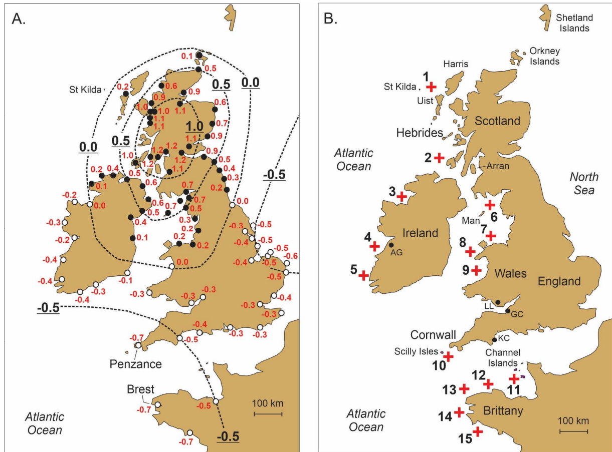
Figure 2. A: Rates (mm/year) of late Holocene relative sea- and land-level changes. Rates for the British Isles are from Kuchar et al. (2012). Rates for Brittany were computed from the ICE 6G GIA model (Peltier et al., 2015). Black-filled circles signify sites that are emerging (the land is rising relative to sea level); open (unfilled) circles signify sites that are being submerged (the land is sinking relative to sea level). B: Locations of the 15 groups of stories presented in Section 3.
