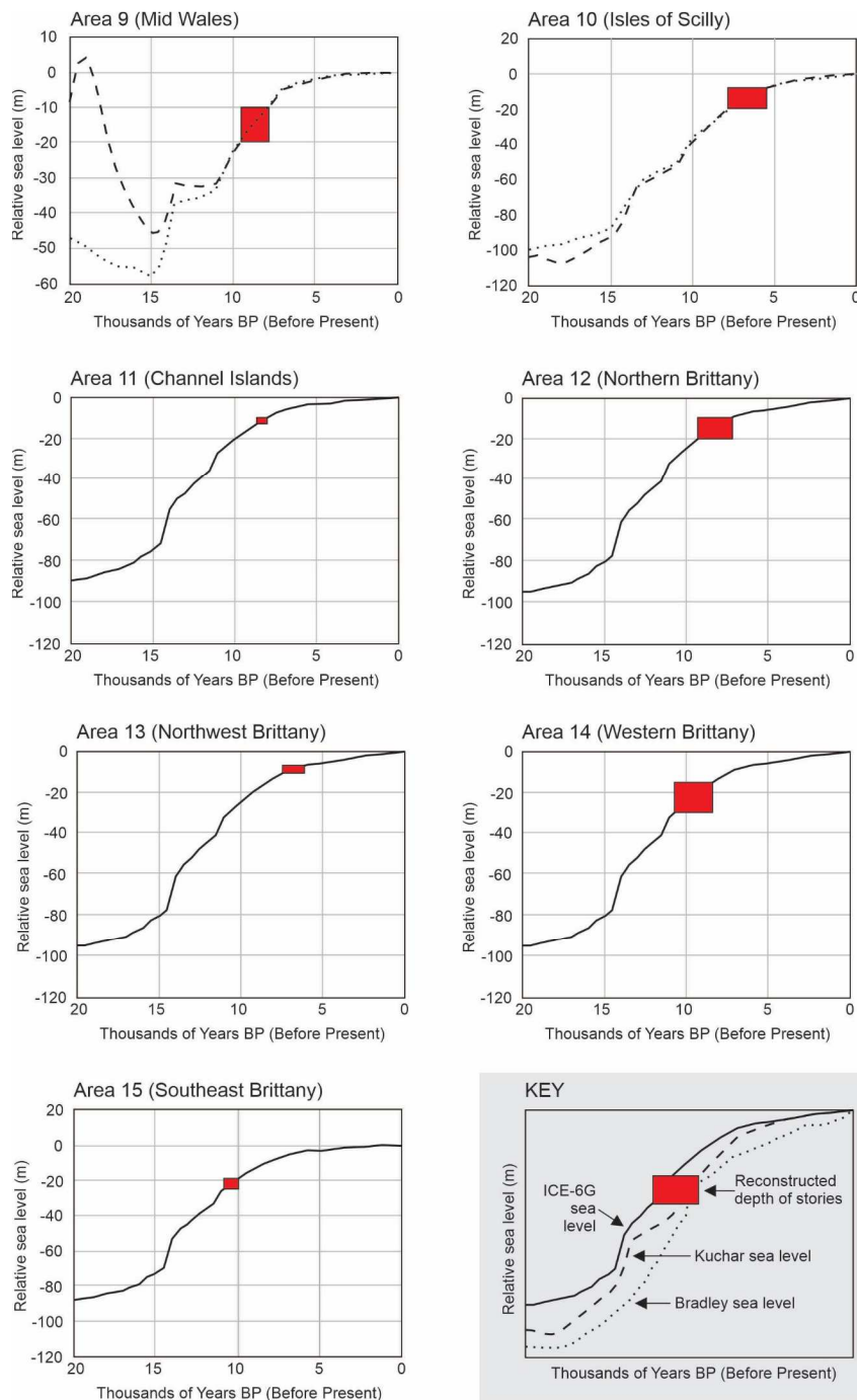
Figure 5 (in two parts). Relative sea-level changes within the past 20,000 years at selected sites within the study region. The Bradley and Kuchar models (Shennan et al., 2018) are considered to be best suited to the British Isles and the ICE-6G data (Peltier et al., 2015) better aligned with Brittany. Shaded (red) boxes represent the estimated depths of coastlines reconstructed from the 15 stories (Table 1). These graphs are used to assign minimum age ranges to these stories (listed in Table 2) and compared to Australian data in Figure 6. Note that the shaded boxes for Areas 2a, 2b and 3 have been assigned an arbitrary 500-year range in the absence of depth-range data.
