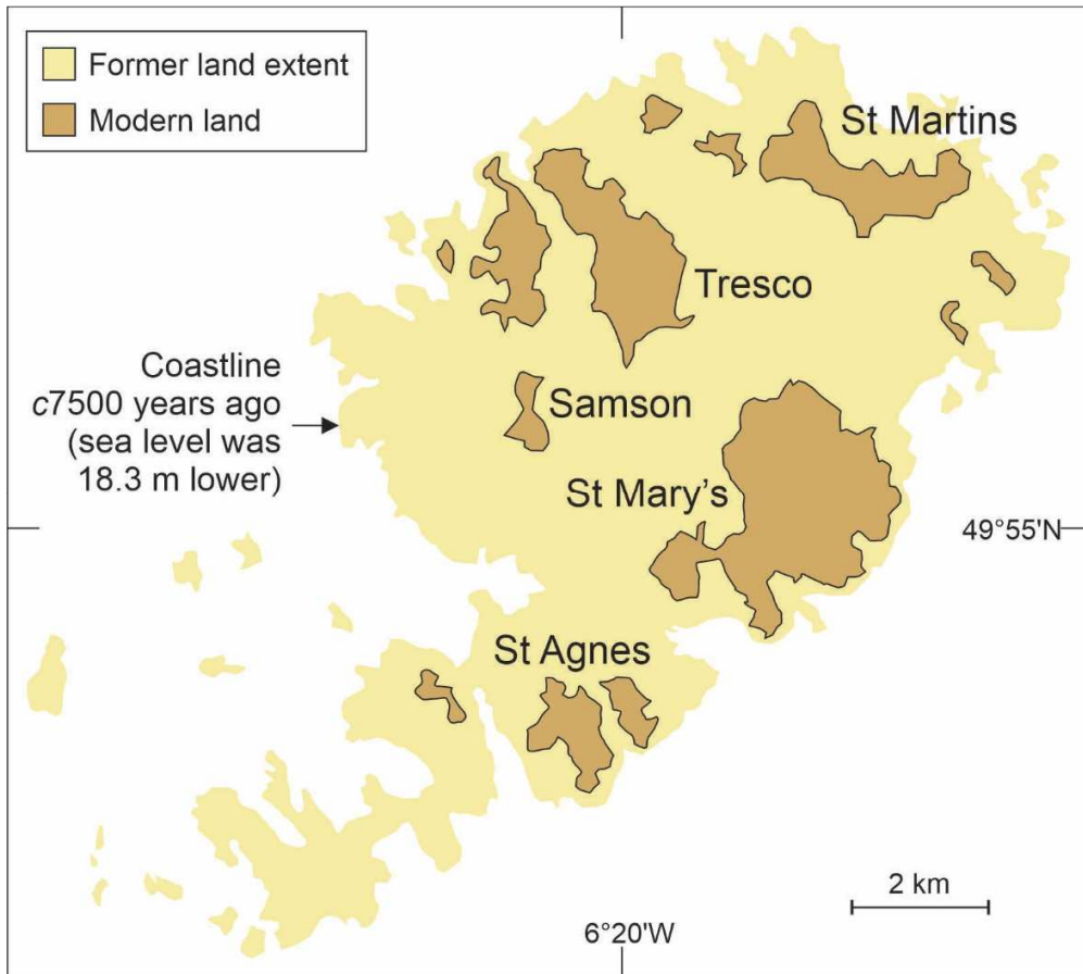
Figure 3. Around 7500 years BP (sea level 18.3 m lower), the Scilly Isles were occupied by people; Mesolithic occupation was c 10,500-6000 years BP (Charman et al., 2016). It is possible that Lyonesse stories originated in the Scilly Isles around this time, not least given the antiquity proposed for similar stories elsewhere (Nunn, 2018).
