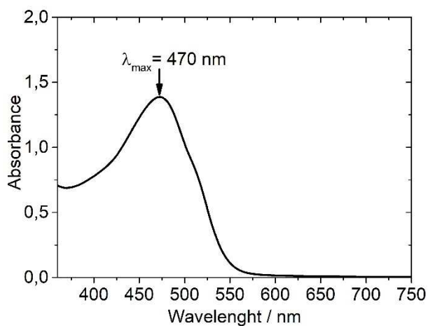
Fig. 7. Absorption UV-visible spectrum of the orange dye G.
