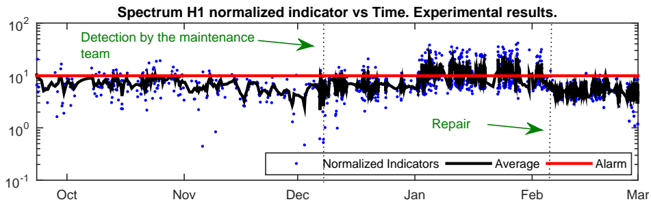
(c) IAS H1 Normalized indicator. Experimental results.
