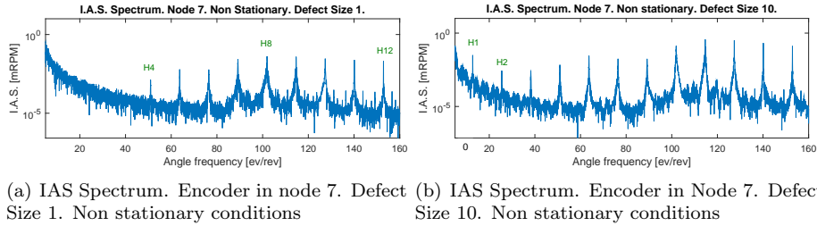
Figure 22: IAS logarithmic spectra in presence of defect sizes 1 and 10. Non stationary conditions.
