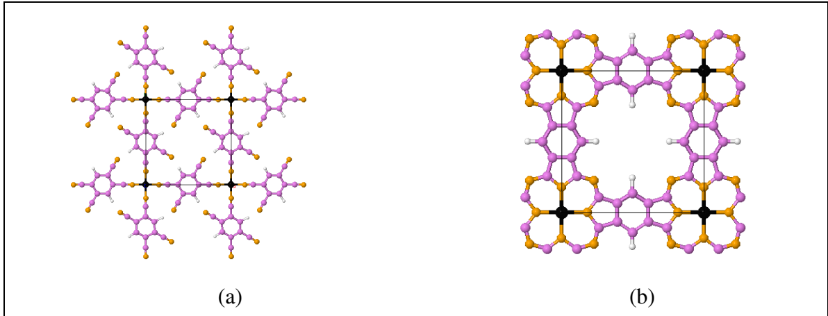
Figure 1. Structures of TM-TCNB metal-organic networks (a) and 2D TM-Pc polymers (b). The TM, N, C, and H atoms are highlighted in black, orange, violet, and white respectively.
