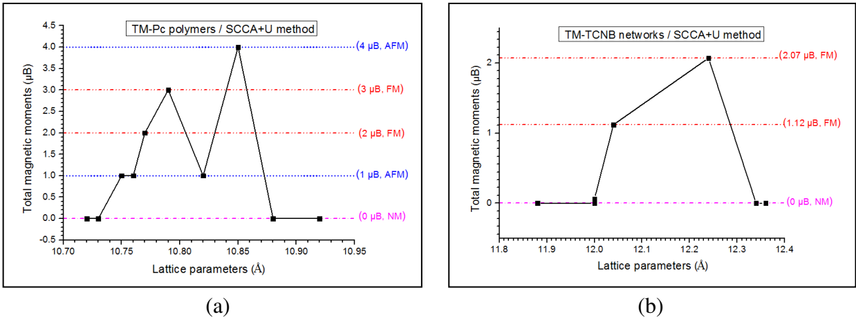
Figure 2. Total magnetic moments ( \mu_B ) as a function of lattice parameters ( \text{\AA} ) for TM-Pc polymers (a) and TM-TCNB materials (b) via SGGA+U approach. The horizontal lines (pink, red, and blue) describe the ground state of structures.
