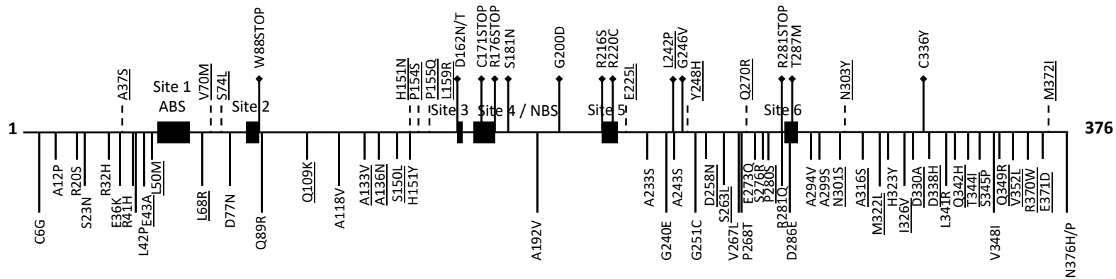
Figure 1. Schematic representation of the UL23 substitutions (amino acids) reported among the 239 HSV1
