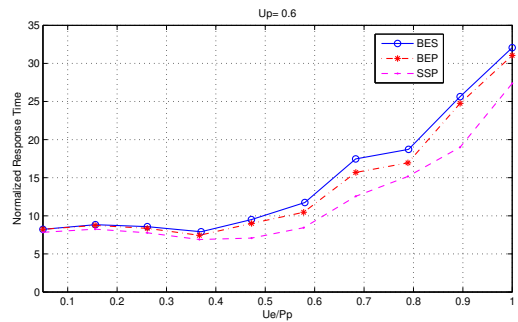
Fig. 5. Aperiodic response time with respect to U_e/P_p , for U_p=0.6 under rectifier signal.
