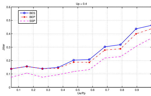
Fig. 7. Jitter time with respect to U_e/P_p , for U_p=0.4 under constant profile.
