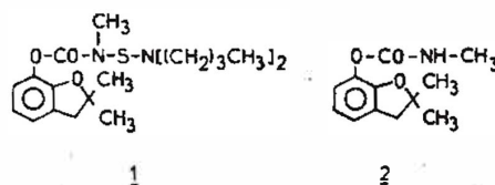
Figure 1. Studied structures: carbosulfan (1) and carbofuran (2).
