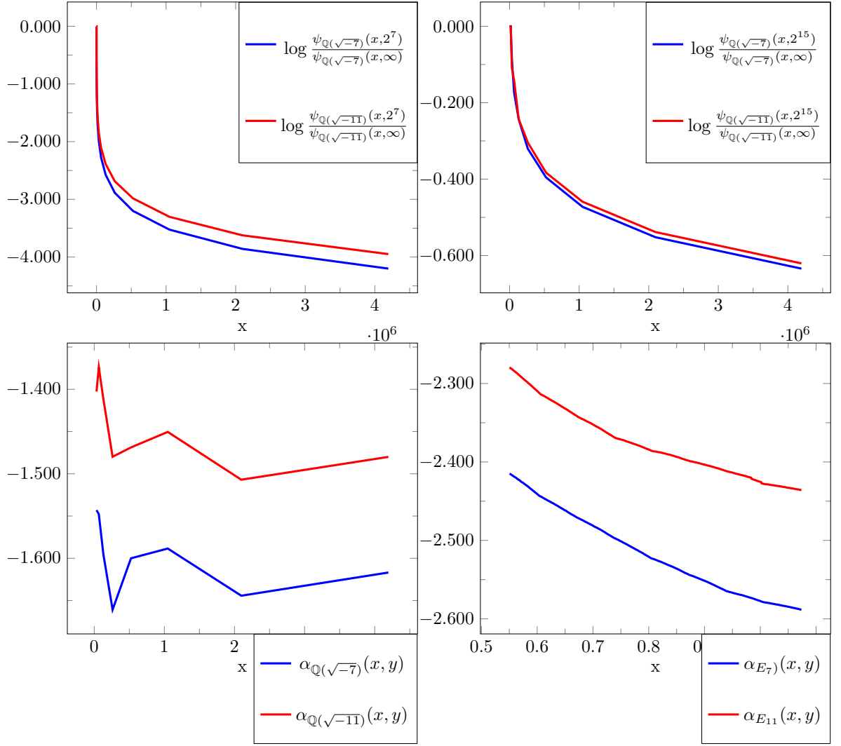
Figure 2: \alpha_K(x, y) := \log\left(\frac{\psi_K(x, y)}{\psi_K(x, \infty)} \frac{\rho(u)^{-1} - 1}{\log(u+1)/\log y}\right) and \alpha_E(x, y) := \log\left(\frac{\psi_E(x, y)}{\psi_E(x, \infty)} \frac{\rho(u)^{-1} - 1}{\log(u+1)/\log y}\right)
