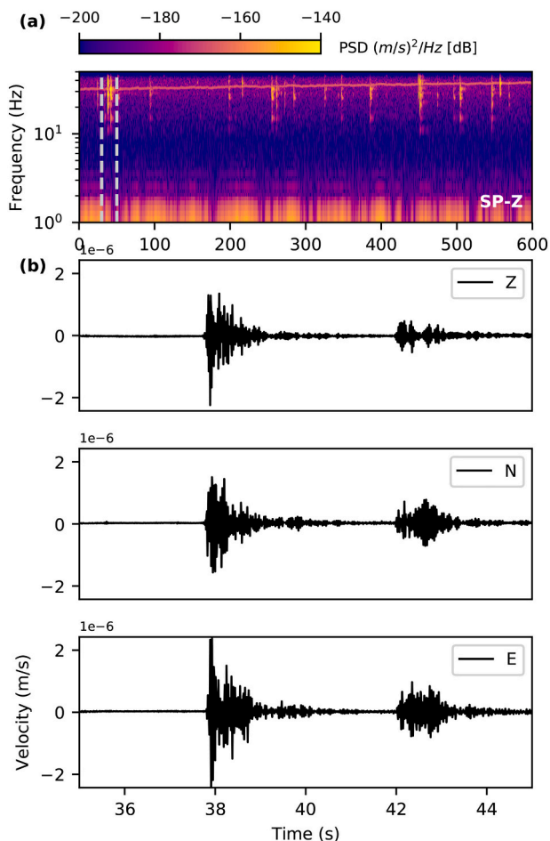
Fig. 5. Donk examples as seen on the 100 sps SP data (channel 65.EH?). (a) Velocity spectrogram for the vertical component, and (b) three component waveform plots for the time frame marked with vertical dashed lines in (a). The time scale in (b) is only 10 s long starting from 2019-07-30 13:36:00 UTC (Sol 239 18:13:42 LMST). Note that donks can be ubiquitous in the data, and have significant variation in amplitude, as well as seismic signal shape and spectral content.
