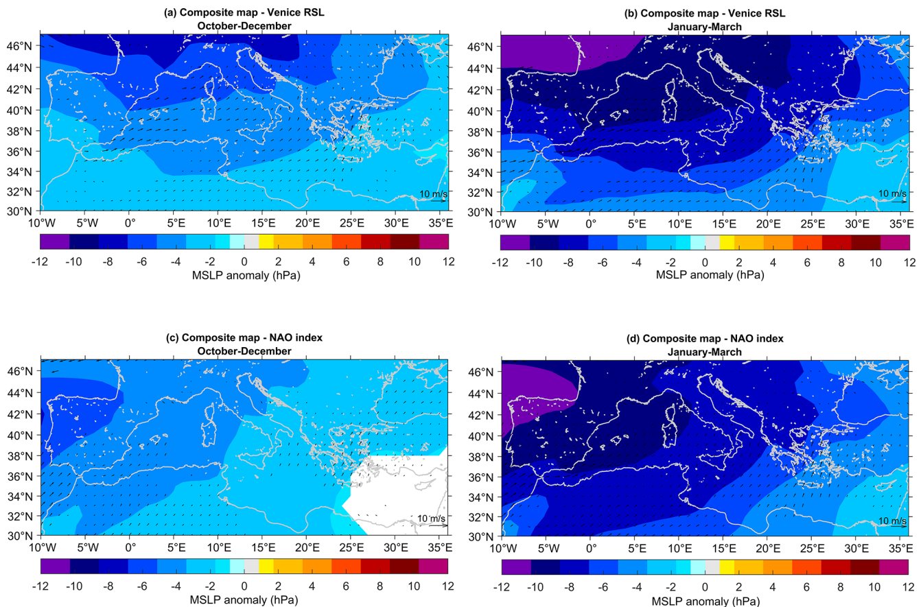
Figure 8. Composite analyses of autumn (OND, a, c ) and winter (JFM, b, d ) reanalyzed mean sea-level pressure (MSLP; shading) and 10 m wind (arrows) around Venetian sea-level ( a, b ) and NAO anomalies ( c, d ). Composite years are determined based on detrended seasonal values of Venetian VLM-corrected RSL (second-order polynomial trend) and of the Jones' NAO index (linear trend) below the 10th percentile and above the 90th percentile. Shown differences are for high minus low sea level ( a, b ) and for negative minus positive NAO ( c, d ). Analysis is for the period 1872–2015 and for linearly detrended sea-level pressure and wind data. Only grid points where differences are significant at 90 % confidence according to the Wilcoxon rank test are shown.
