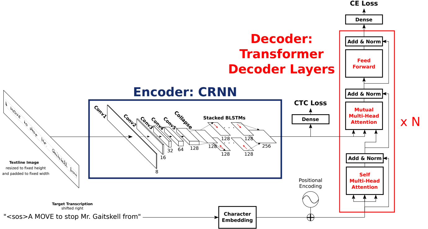
Figure 2. Our Sequence-to-Sequence Transformer Model
