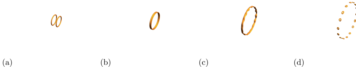
Figure 3. Snapshots for the instability of two colliding vortex rings. The initial condition consists of two vortex rings of the same radii: R = 12.4 \pm 0.5 units. (a) The two vortex rings drifting head-on, (b) vortex rings approaching with the subsequent stretching of the circular filament, (c) the modulational instability and (d) vortex reconnection into 16 smaller vortex rings drifting into the orthogonal plane. The time sequence is (a) t = 160 , (b) t = 220 , (c) t = 250 and (d) t = 270 . The three dimensional surface plot shows the iso-surface of |\psi|^2 = 0.5 . The simulations evolved into a cubic lattice of N = 256^3 with a mesh size dx = 0.5 and a time step dt = 0.01 .
