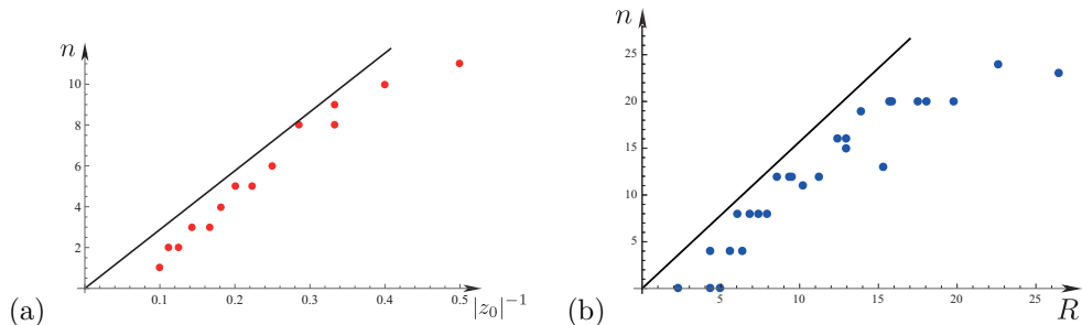
Figure 2. (a) Number of vortex rings as a function of the inverse of the initial distance z_0 . As a visual guide the line represents: n = \frac{\sqrt{2}L}{2\pi} \frac{1}{|z_0|} (See Sec. 2 for the theoretical justification). The initial separation distances are such that |z_0| \in [2, 10] . The upper bound, 10, being the largest separation distance that can be allowed by the modulational instability because one gets just a single loop at the end. (b) Number of vortex rings after the collision of two circular vortex rings colliding head-on. The line represents n = \frac{\pi R}{2} . All simulations were done into a cubic lattice of N = 256^3 with a mesh size dx = 0.5 and a time step dt = 0.01 .
