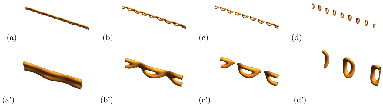
Figure 1. Snapshots of the anatomy of vortex reconnection by the Crow instability mechanism. The initial separation distance was 3 units of length. (a) A modulational instability starts to develop, in (b) it is shown the fore vortex-reconnection instant, (c) shows the after vortex-reconnection instant, and (d) shows the further evolution of 8 drifting vortex rings. The time sequence is (a) t = 30 , (b) t = 38 , (c) t = 40 and (d) t = 50 . The second row plots a zoom of the same time sequence. The three dimensional surface plot shows the iso-surface |\psi|^2 = 0.4 and the simulations evolved into a cubic lattice of N = 256^3 with a mesh size dx = 0.5 (length units) and time step dt = 0.01 .
