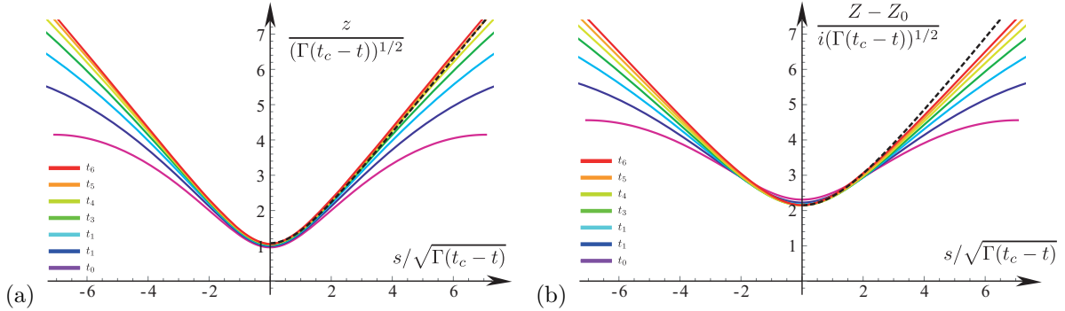
Figure 5. Self-similar evolution of the re-scaled functions (10,11) as a function of the self-similar variable \omega = s/\sqrt{\Gamma(t_c - t)} . (a) Plots z/\sqrt{\Gamma(t_c - t)} vs \omega and (b) -i(Z - Z_0)/\sqrt{\Gamma(t_c - t)} vs \omega . The segmented black line represents the solution of (13) and (14) with boundary conditions (15) and matching condition (22).
