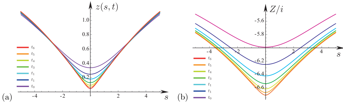
Figure 4. Time evolution of the vortex filament variables z(s, t) and Z(s, t) . (a) Plot of z(s, t) for different time steps. (b) Plot of Z(s, t) for same time steps as in (a). The simulations were done for L = 10 , an initial perturbation of the form (9) with z_0 = 4 and \epsilon = 0.1 getting a finite time singularity at a time with t_c \approx 44.756 . With initial condition (9) one has t_c \approx 44.756 and Z_0 \approx -27.223 i . The time steps are t_n = t_c - 2^{1-n} .
