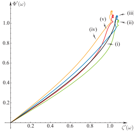
Figure 6. \Phi' - \zeta' projection of the trajectories, five different trajectories are shown for parameters (a_0, b_0) taking the following values: (i) (1.071, 2.125); (ii) (1.044, 2.088); (iii) (1.106, 2.088); (iv) (1.044, 2.213); (v) (1.106, 2.213).
