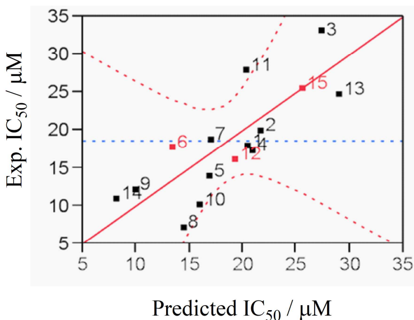
Figure 3: Correlation of experimental and predicted IC_{50} (in \mu M ) as derived using MLR.
