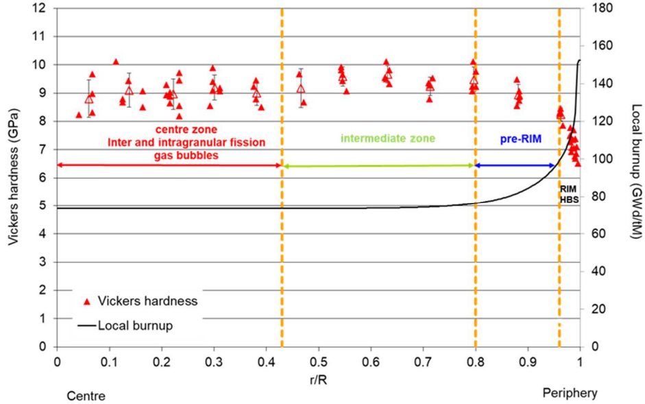
Fig. 9. Vickers hardness (indentation load 0.735 N) and local burnup of the irradiated standard \text{UO}_2 – 81.6 GWd/tm as a function of the radial position. The local burnup was deduced from the neodymium content, measured by EPMA. The single hardness values are indicated by solid triangles and the average value of hardness at 12 radial positions is indicated by empty triangles. In the pre-rim zone, the fuel is partially in the HBS and in the rim zone, the fuel is totally in the HBS.
