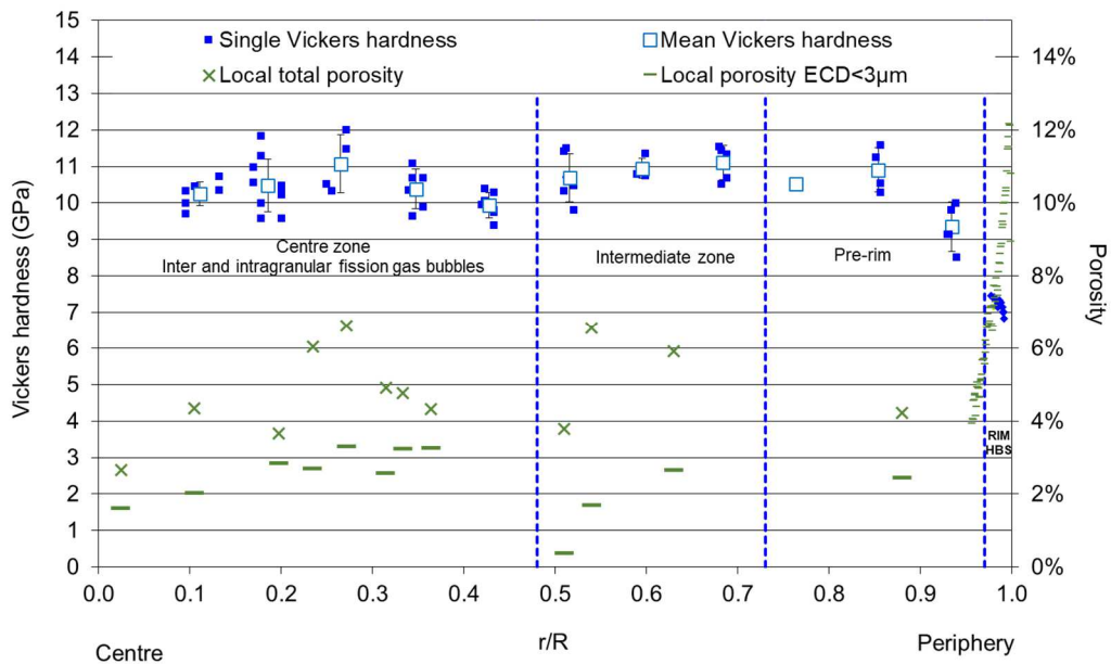
Fig. 10: Vickers hardness (indentation load 0.735 N) and local porosity (total and ECD < 3 \mu\text{m} ) of the irradiated doped \text{UO}_2 – 60.8 GWd/tm as a function of the radial position. The local porosity was determined by SEM images analysis. The single hardness values are indicated by blue solid squares and the average value of hardness at 11 radial positions is indicated by blue empty squares. Inter-granular and intra-granular fission gas bubbles are precipitated in the centre zone. The
