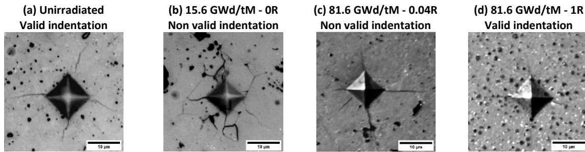
Fig. 5. Indentations in unirradiated and different irradiated standard \text{UO}_2 fuels (indentation load 0.735 N).
