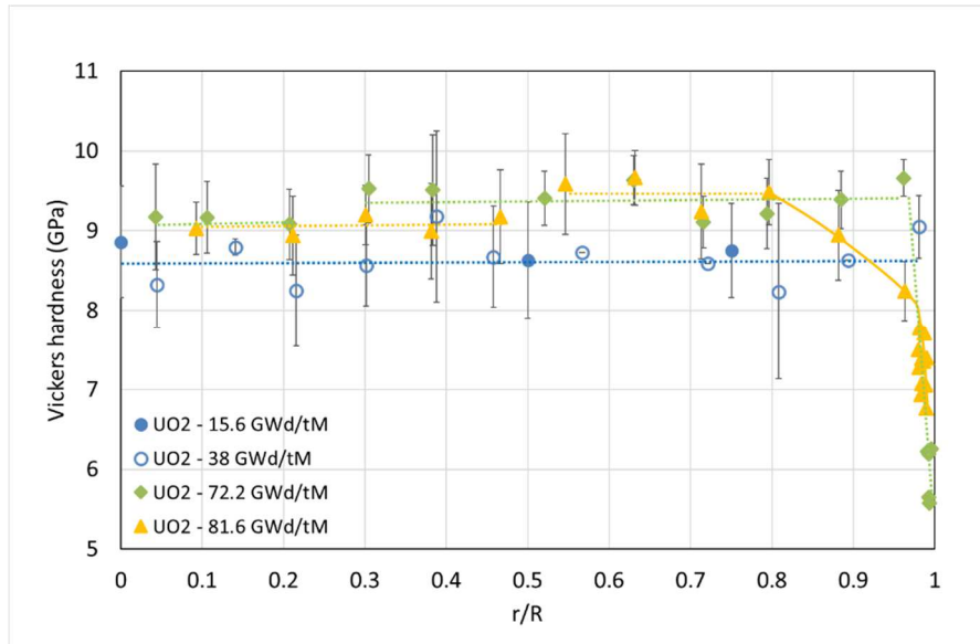
Fig. 16. Evolution of the Vickers hardness profiles of standard \text{UO}_2 fuels with the average burnup of the pellet (indentation load 0.735 N).
