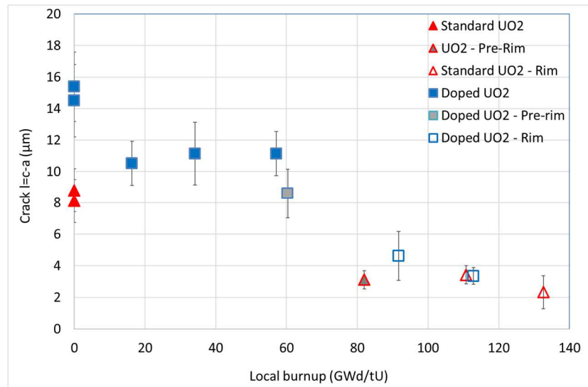
Fig. 11. Crack length l in standard \text{UO}_2 and doped \text{UO}_2 as a function of the local burnup (indentation load
