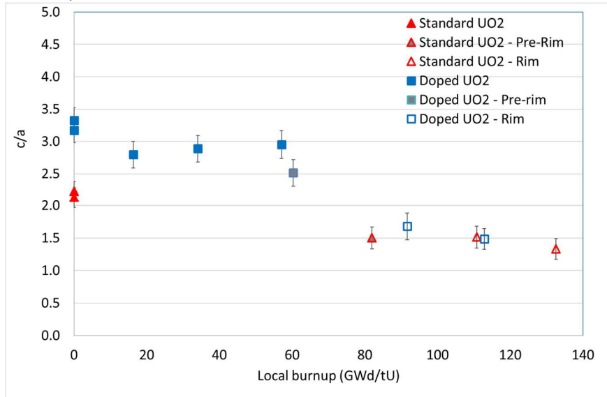
Fig. 13. Ratio c/a as a function of the local burnup for the standard \text{UO}_2 and the doped \text{UO}_2 (indentation load 0.735 N). For the high burnups fuels >50 GWd/tM, the pre-rim and rim zones of the pellet are indicated in the legend ; otherwise, the fuels come from the centre and the intermediate zones ( r/R < 0.8 ).
