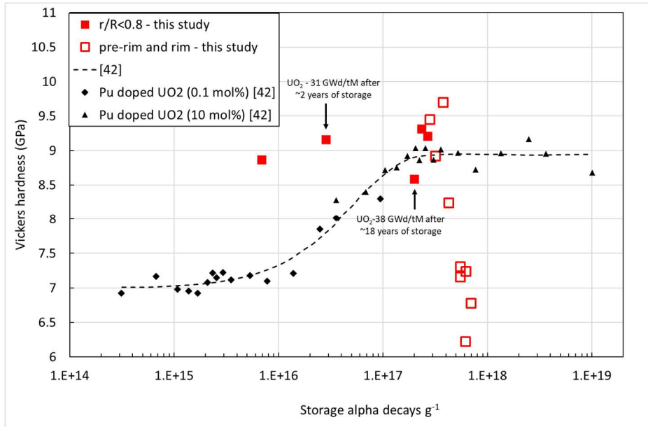
Fig. 17. Vickers hardness as a function of alpha decay densities. In this study, the \text{UO}_2 samples were irradiated in a reactor at different burnups. The alpha decays were calculated during storage time with the Prodhel model [43]. The [42], unirradiated Pu doped \text{UO}_2 samples accumulated alpha dose during their storage
