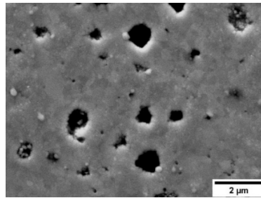
Fig. 2. SEM micrograph of HBS – Doped \text{UO}_2 fuel – 60.8 GWd/tM
