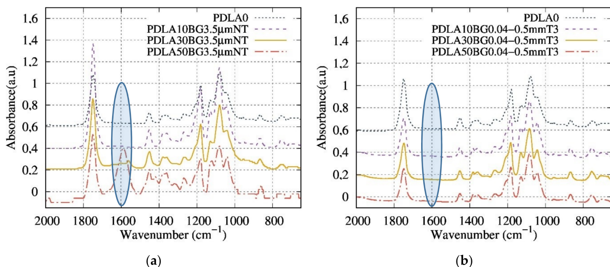
Figure 5. Superposition of (a) FTIR spectra of composites containing various contents of BG 3.5 μm NT (wt%); (b) FTIR spectra of composites containing various contents of BG 0.04–0.5 mm T3 (wt%).
