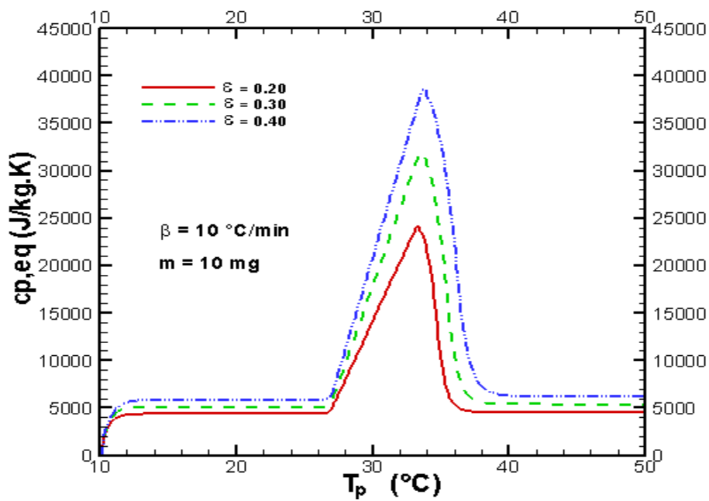
Fig.18-c: Equivalent heat capacity versus T_p for various \epsilon
