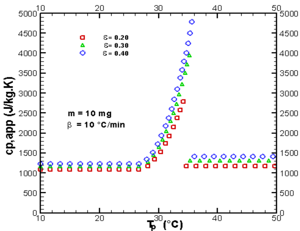
Fig.18-b: Apparent heat capacity versus T_p for various \epsilon
