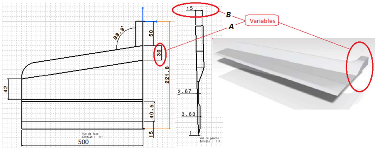
FIGURE 17. Geometry of the flat die.
