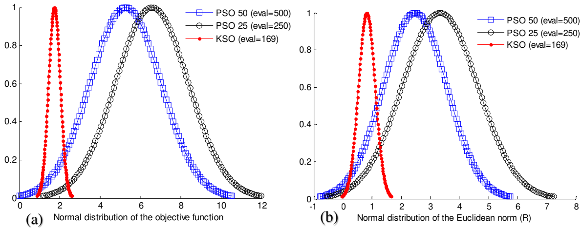
FIGURE 8. Normal distribution plot based on the best objective function (a) and Euclidean norm (b) values for 4d Ackley function.
