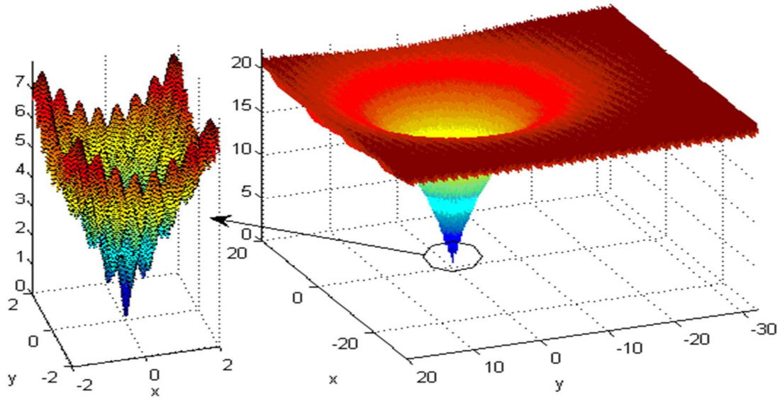
FIGURE 6. Two-dimensional illustration of Ackley function
