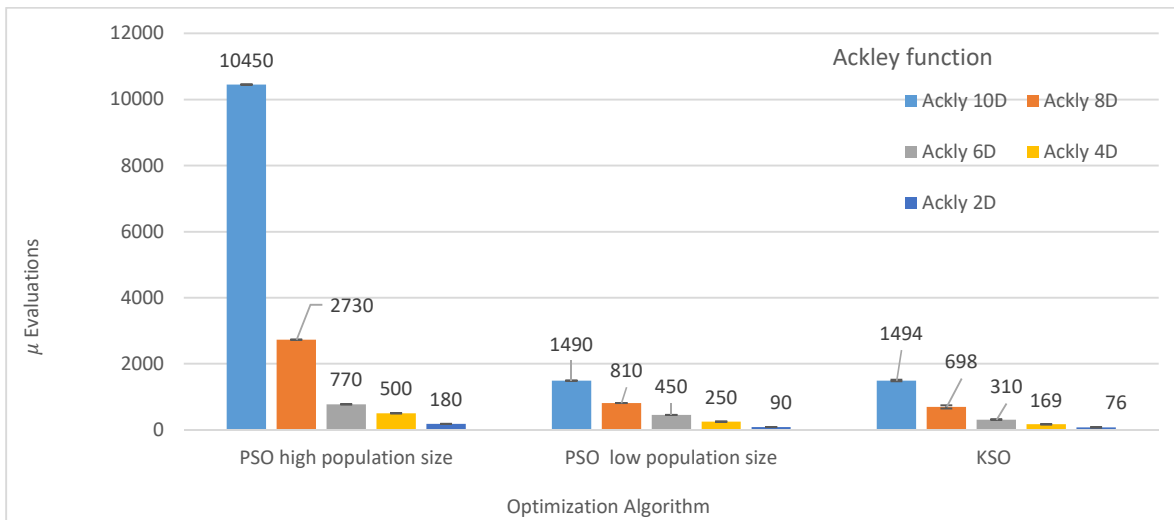
FIGURE 16. Mean plot of function evaluations for d dimension Ackley problem.
