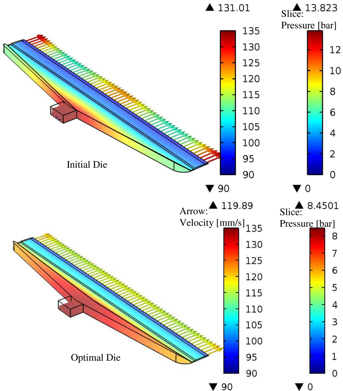
FIGURE 21. Pressure distribution in initial and optimal dies.
