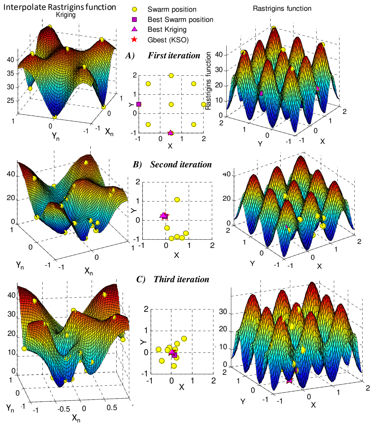
FIGURE 3. An illustration of metamodels according to Kriging method based on PSO and SDB for each iteration.
