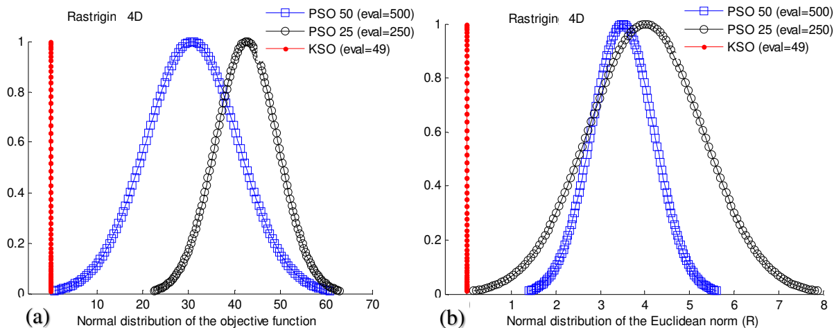
FIGURE 10. Normal distribution plot based on the best objective function ( f ) and Euclidean norm ( R ) values for 4d Rastrigin function.
