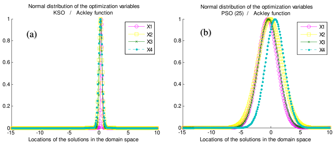
FIGURE 7. Normal distribution plot based on the best solution values of the optimization variables for both KSO (a) and PSO (b) algorithm for 4d Ackley function.
