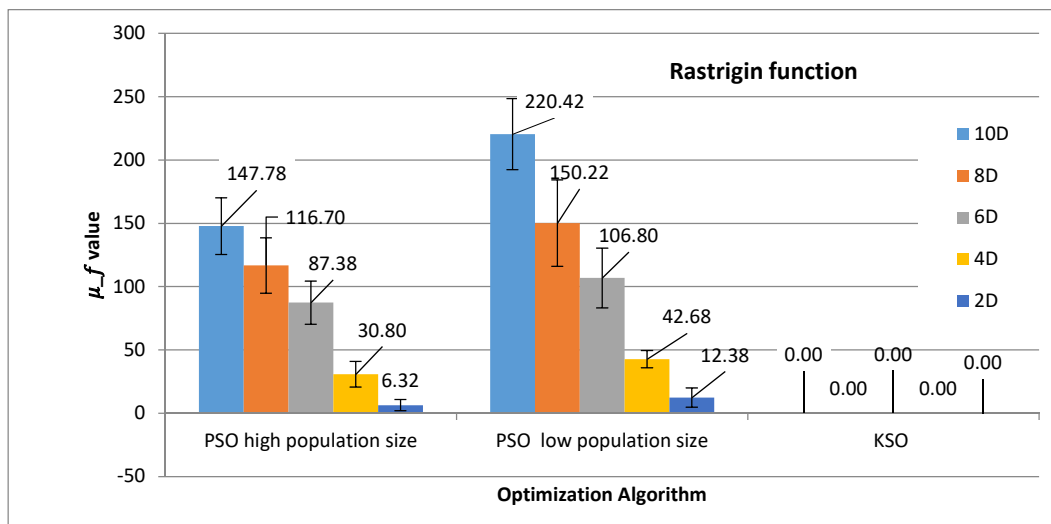
FIGURE 13. Mean and quartile plot of objective function values for d dimension Rastrigin problem.
