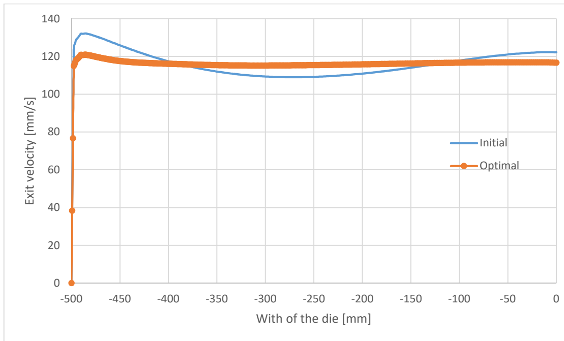
FIGURE 19. Exit velocity distribution in mid plane for initial and optimal die.
