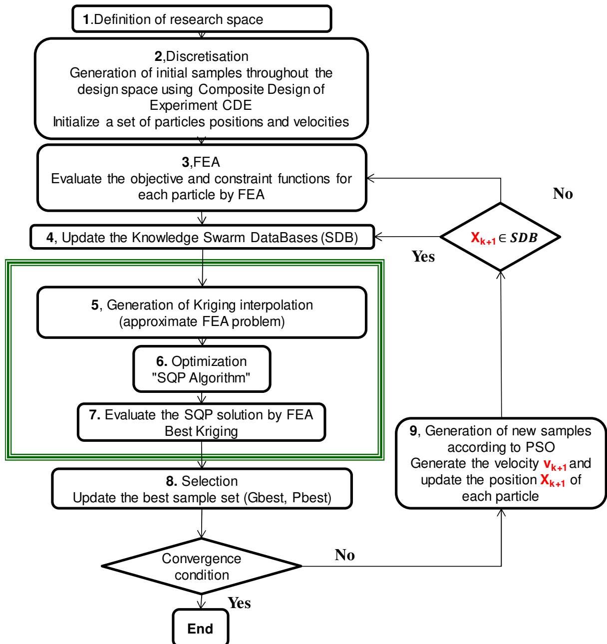
Figure 1. Flow-chart of KSO Algorithm.
