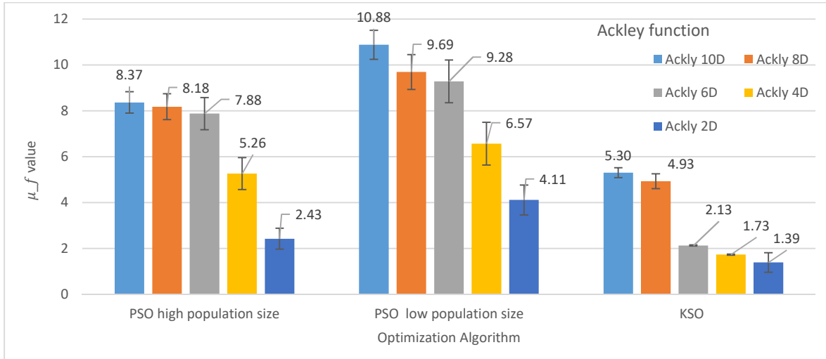
FIGURE 15. Mean and quartile plot of objective function values for d dimension Ackley problem.
