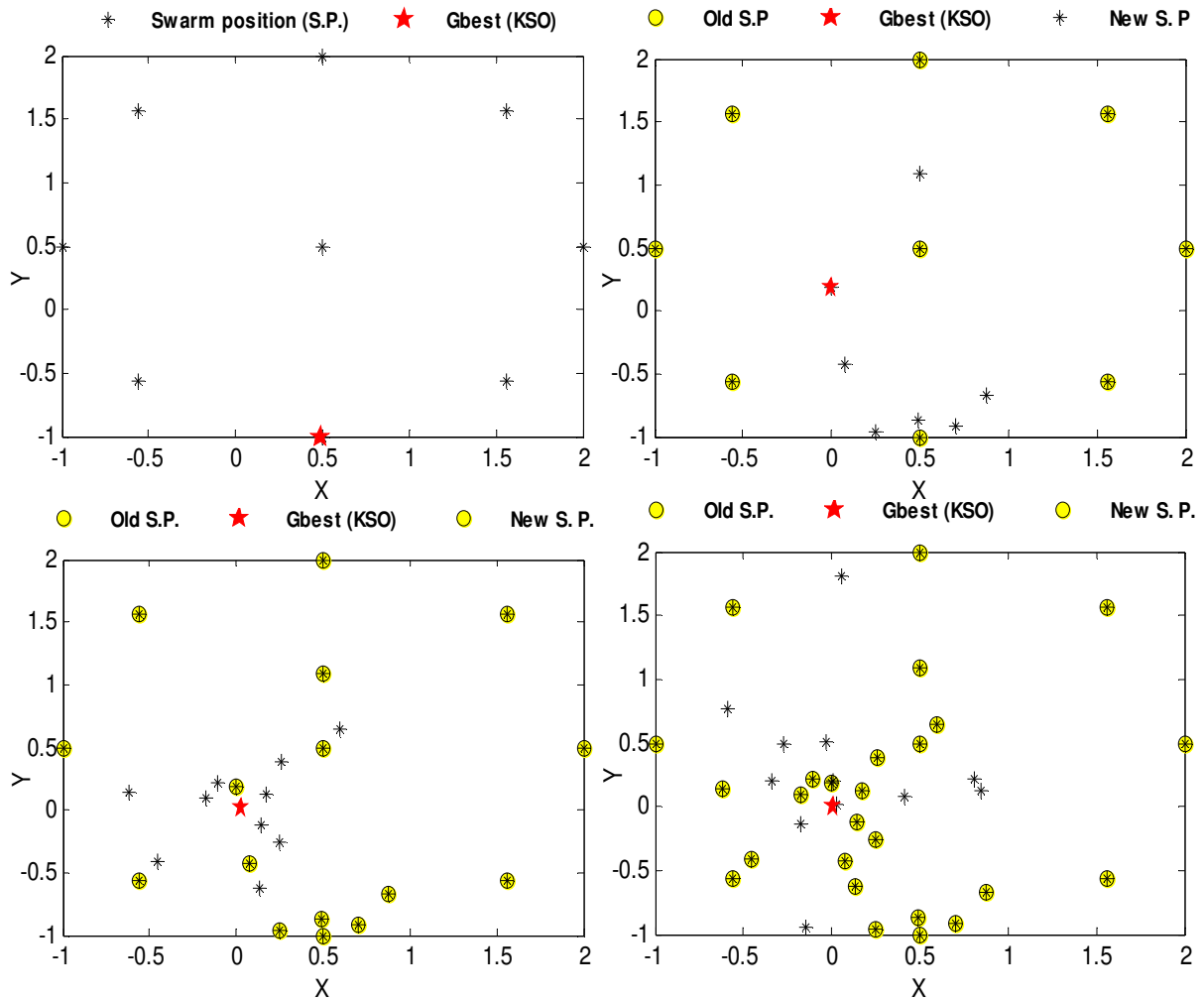
FIGURE 4. An illustration of samples distribution generated by PSO and SDB for each iteration
