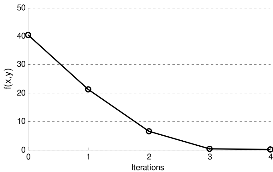
FIGURE 5. Convergence history of the optimization of Rastrigin function
