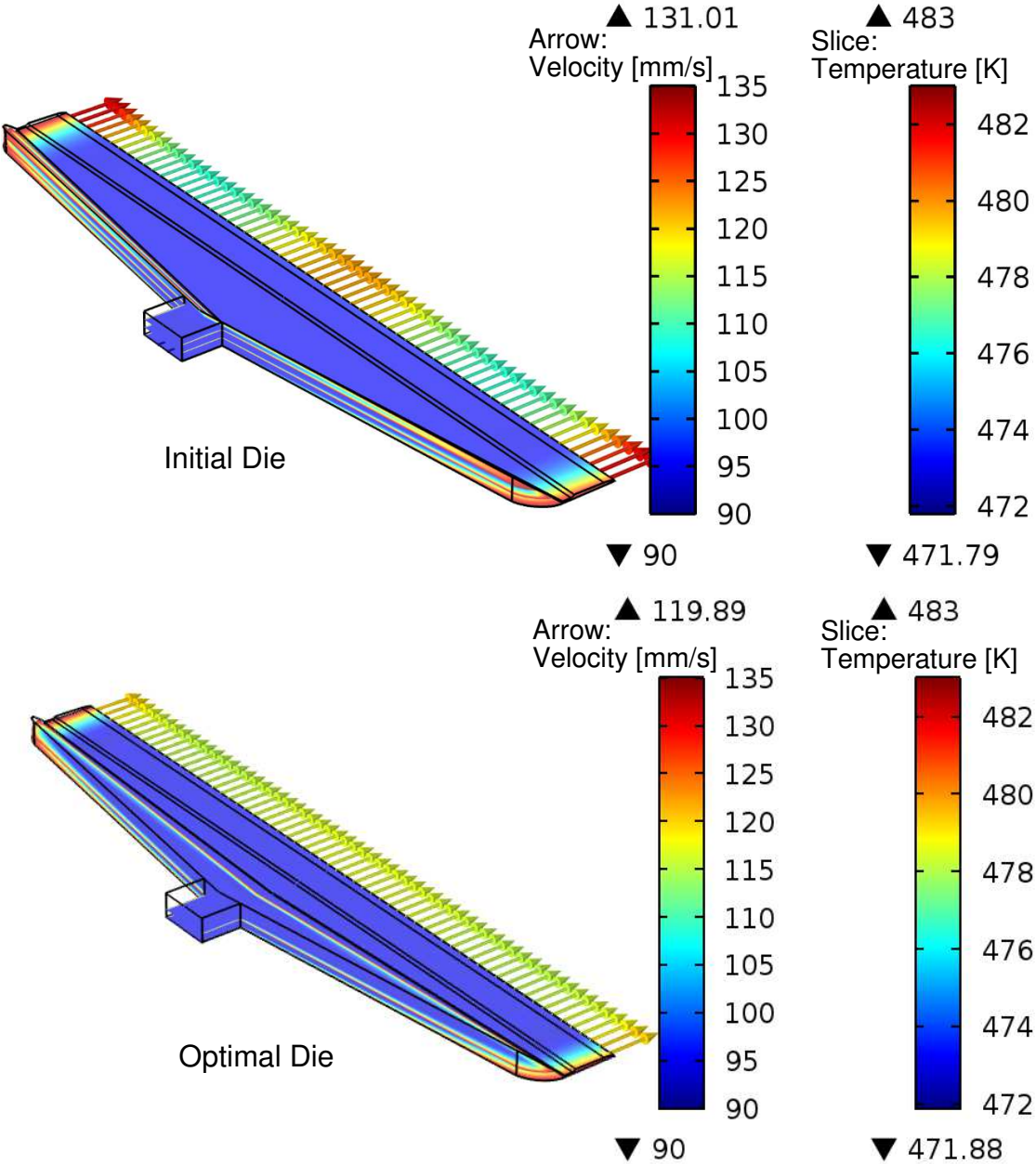
FIGURE 22. Temperature distribution in initial and optimal dies.
