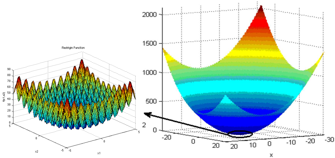
FIGURE 9. Two-dimensional illustration of Rastrigin function
