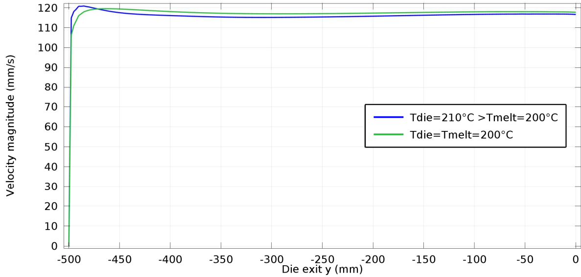
FIGURE 23. Effect of die temperature on the optimal velocity distribution.
