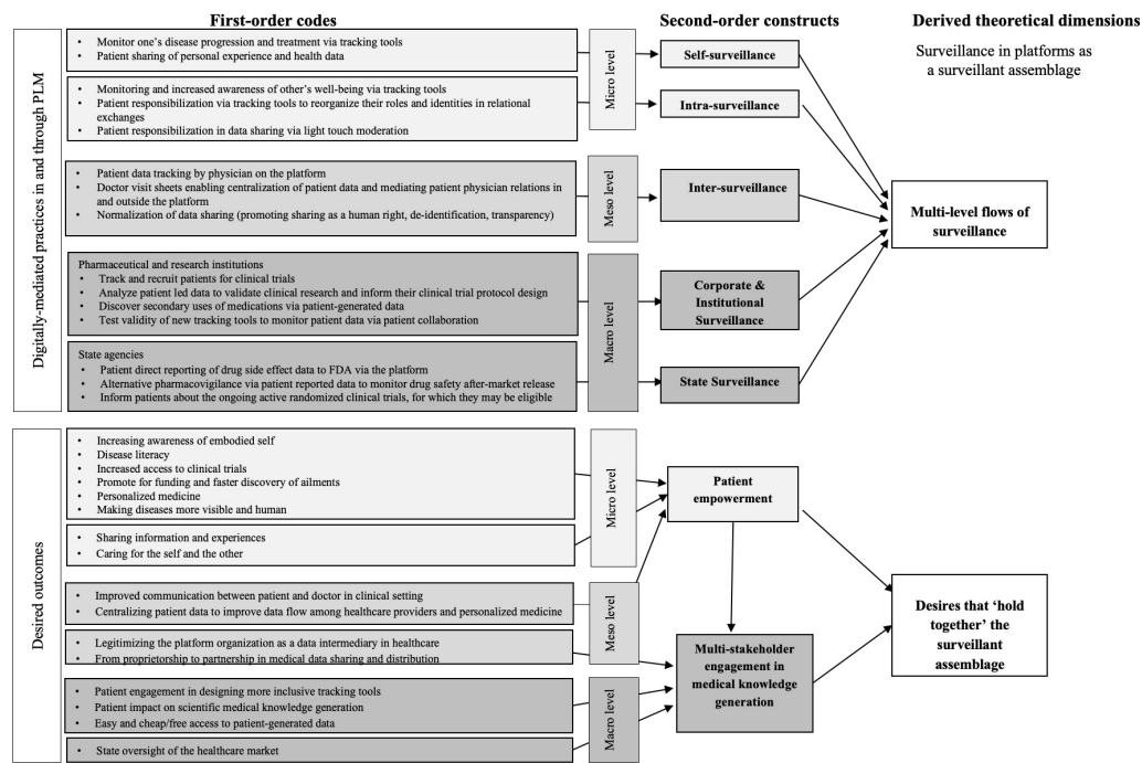
FIGURE 1 DATA STRUCTURE
