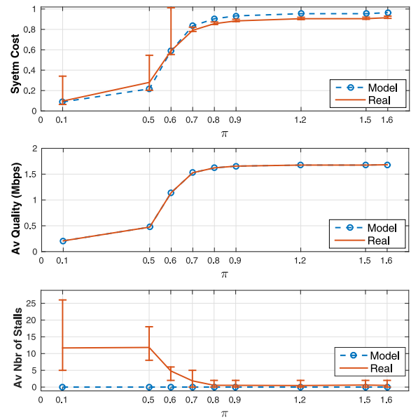
Fig. 21. NEWCAST performance in real environment.
