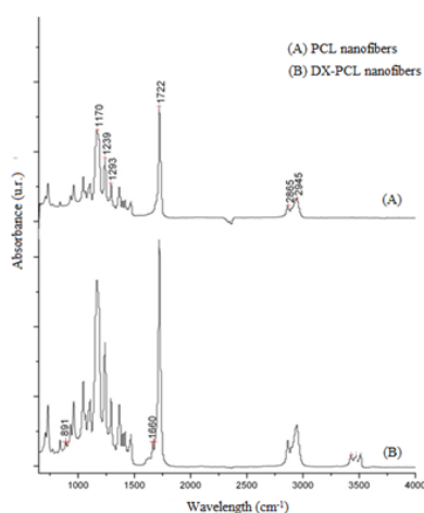
Figure 2. FTIR spectra of PCL nanofibers (A) and DX PCL nanofibers (B).
