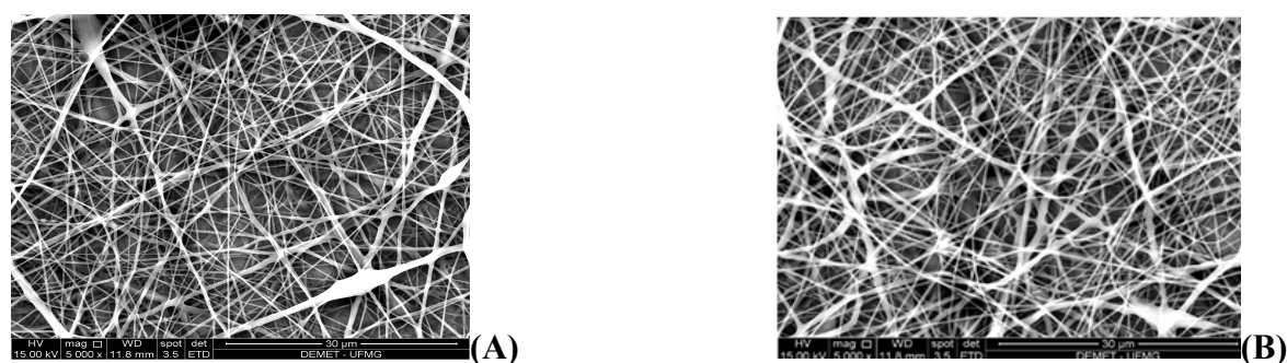
Figure 1. SEM photomicrograph of PCL nanofibers (A) and DX PCL nanofibers (B). Magnification - 5000×. Scale bar – 30 μm.
