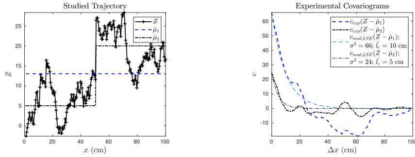
Figure 1: Experimental covariograms for different assessments of the mean : case of a non-stationary trajectory
