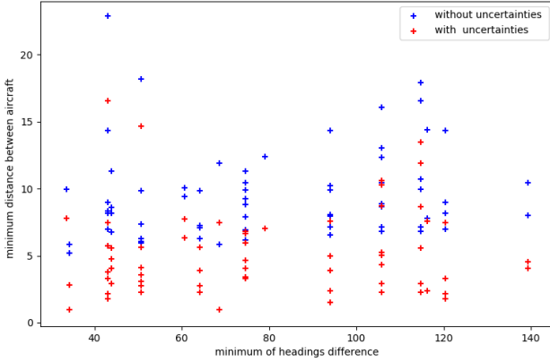
Fig. 12: Three aircraft experiments : Minimum separation distance between aircraft with and without uncertainties
