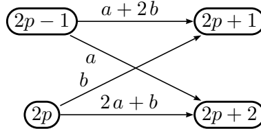
Figure 4. The transitions of the Railroad \mathbb{Z} -automaton
