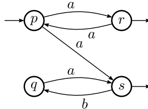
Figure 3. The nondeterministic automaton \mathcal{A}_2
