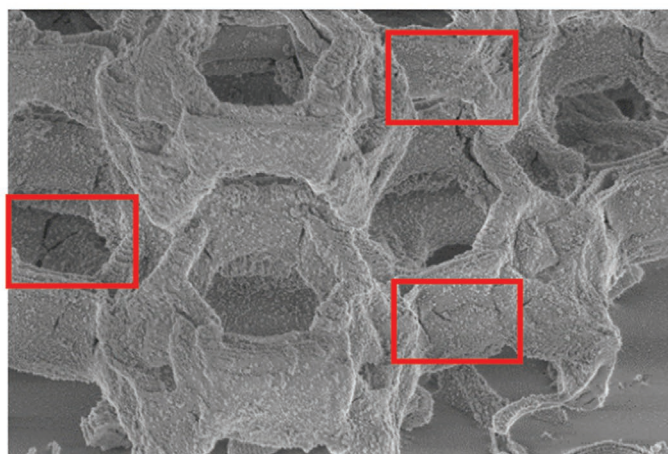
(b) Cracks within the sintered structure
