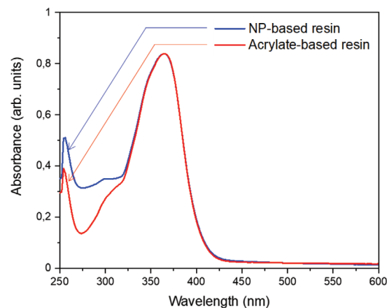
Figure 3. UV-vis absorption spectra of the two resins (diluted 10 000 times in ethanol).
