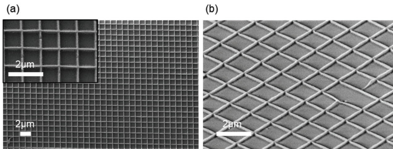
Figure 14. Pyrolyzed microgrid with a period of 1 \mu\text{m} : a) view from the top b) view with 45° tilt.
