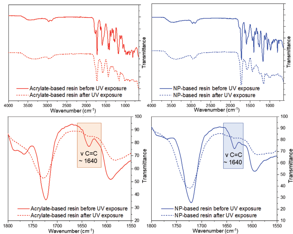
Figure 5. FTIR spectra of both resins before and after UV exposure in the range 650–4000 cm -1 and zooms on the C=C elongation at 1640 cm -1 .
