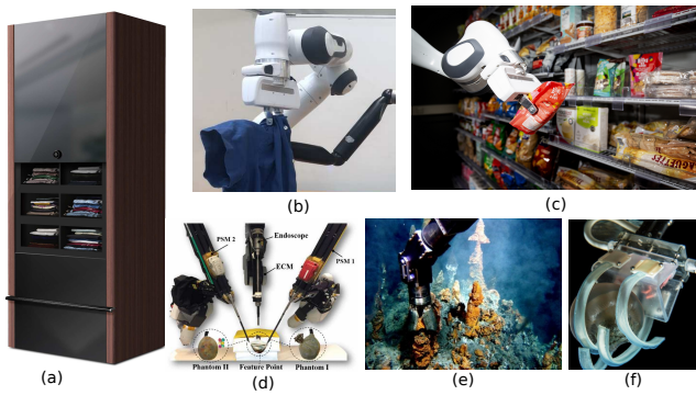
Fig. 6. Various applications of DOM – (a): laundry-folding robot from Seven Dreamers Laboratories Inc. [81], (b): A mock-up for robotics dressing assistance, (c): a robot picking a flexible bag of goods on the shelf, courtesy AIR-Lab Delft [82], (d): autonomous surgical manipulation by the dVRK system [83], (e): ROV Victor 6000 sampling black smokers (IFREMER/GENAVIR) courtesy D. Desbryères, (f): Ultra soft underwater gripper for jellyfish [84]
