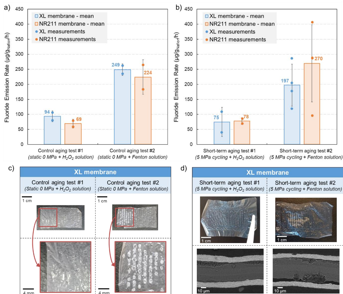
Fig. 2 – Fluoride emission rates (FER) of Nafion ™ XL and NR211 membranes under (a) static 0 MPa and (b) cyclic 5 MPa compressive stress coupled to moderate ( \text{H}_2\text{O}_2 solution) and aggressive (Fenton solution) chemical stress. FER presented in Figure 2b correspond to data already published in a previous work [39] that have been corrected in this study by subtracting a parasitic contribution in fluoride concentration coming from the TISAB II solution employed for measurements. (c) and (d) illustrate the evolution of the XL membrane morphology at
