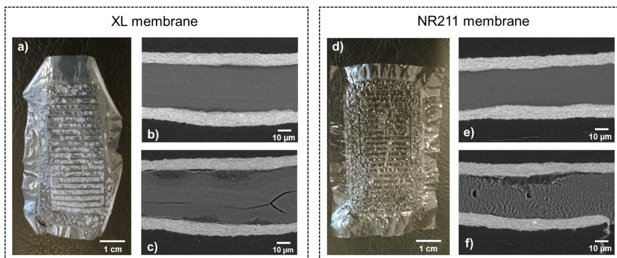
Fig. 5 – Macroscopic surface morphology of Nafion ™ (a) XL and (d) NR211 membranes after long-term aging test and comparison of SEM cross-sections for pristine and aged (b, c) XL and (e, f) NR211 membranes. SEM images were performed on MEA made with aged membranes and after conducting the electrochemical tests in single cell (more details are given in section 2.4.5).
