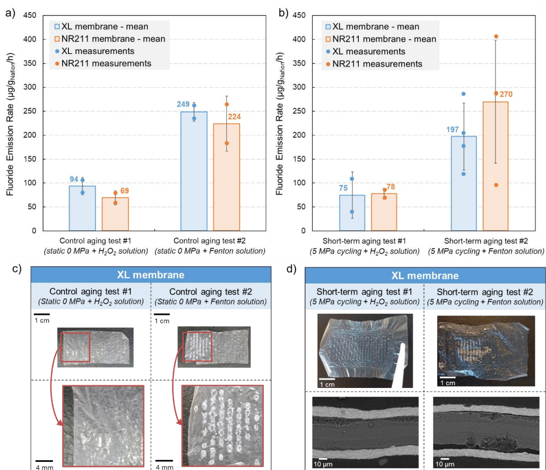
Fig. 2 – Fluoride emission rates (FER) of Nafion™ XL and NR211 membranes under (a) static 0 MPa and (b) cyclic 5 MPa compressive stress coupled to moderate (H 2 O 2 solution) and aggressive (Fenton solution) chemical stress. FER presented in Figure 2b correspond to data already published in a previous work [39] that have been corrected in this study by subtracting a parasitic contribution in fluoride concentration coming from the TISAB II solution employed for measurements. (c) and (d) illustrate the evolution of the XL membrane morphology at different scales after the various aging tests. It is noteworthy that SEM images were not acquired in specific area (i.e. in the bubbles area) but taken randomly through the membranes cross-section.
