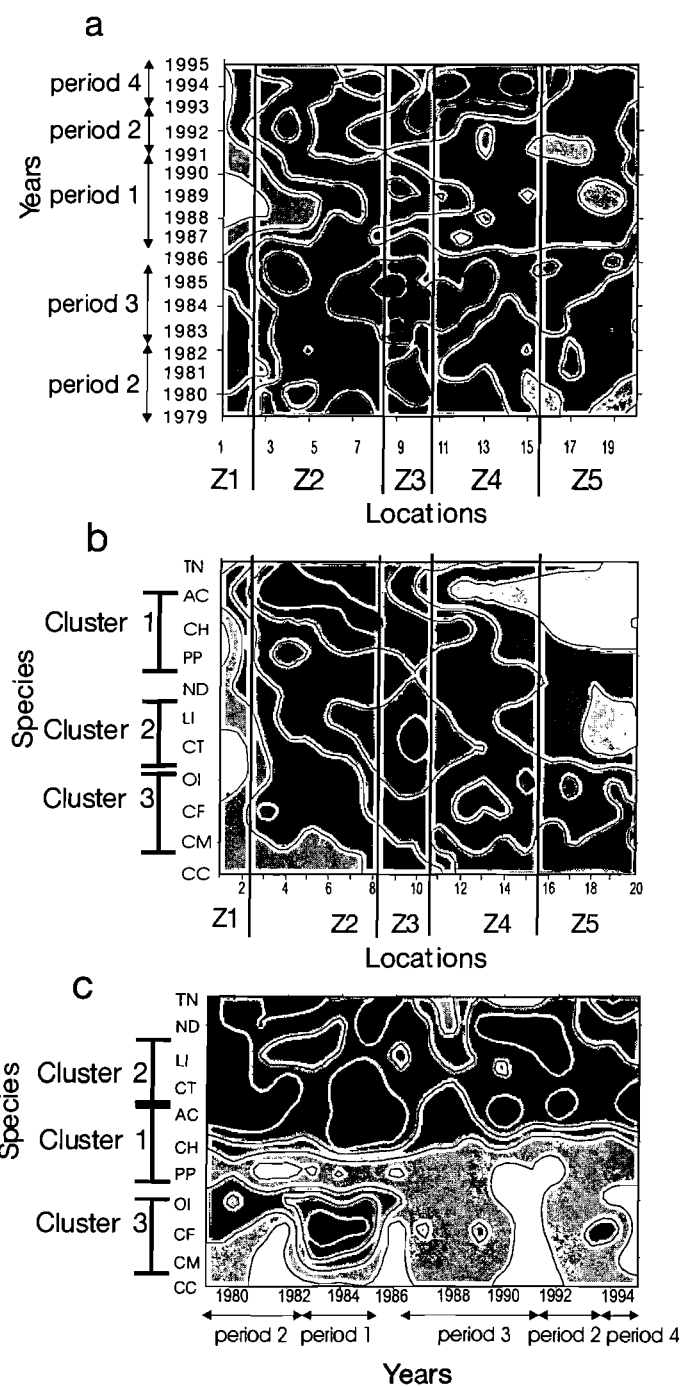
Fig. 4. Year-to-year variability. (a) Species mode ( R^p ). Variability of the first principal component year-location. The grey shading indicates the intensity of the first component. The groups determined from the cluster analysis are indicated for years on the ordinate and for locations on the abscissa. (b) Year mode ( R^t ). Variability of the first principal component species-location. The groups determined from the cluster analysis are indicated for species on the ordinate and for locations on the abscissa. (c) location mode ( R^s ). Variability of the first principal component species-year. The groups determined from the cluster analysis are indicated for species on the ordinate and for years on the abscissa. Z1: northeastern English Channel; Z2: southwestern English Channel; Z3: Ushant Front; Z4: Celtic Sea; Z5: Bay of Biscay. TN: Thalassionema nitzschioides ; AC: Acartia spp.; CH: Calanus helgolandicus ; PP: Para-Pseudocalanus spp.; ND: Nitzschia delicatissima ; LI: Limacina sp.; CT: Centropages typicus ; OI: Oithona spp.; CF: Ceratium fusus ; CM: Ceratium macroceros ; CC: Clausocalanus spp.
