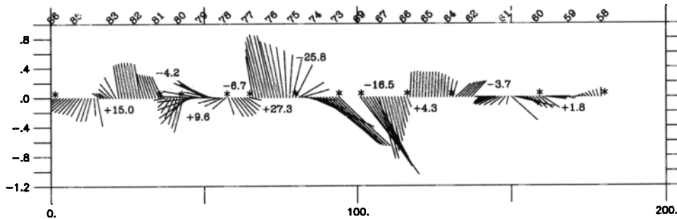
Figure 3. ADCP currents in \text{ms}^{-1} (subsamped every 5 km) and mass transport (15–1800 dbar) in Sv from west (left) to east (right), along the ship trajectory. The transports were calculated from pair of CTD stations, the location of which is indicated by stars. A positive (negative) sign means a northwestward (southeastward) transport relative to the NE–SW ship trajectory.
