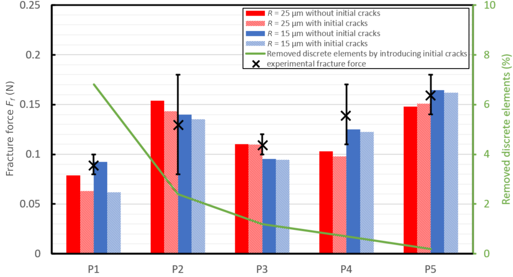
Figure 10: Fracture force for each simulated particle (P1-P5) with and without initial cracks introduced in the coarse ( 25 \mu\text{m} ) and fine ( 15 \mu\text{m} ) discrete elements mesh. The fraction of removed discrete element due to initial cracks introduction is plotted on the right hand side axis.
