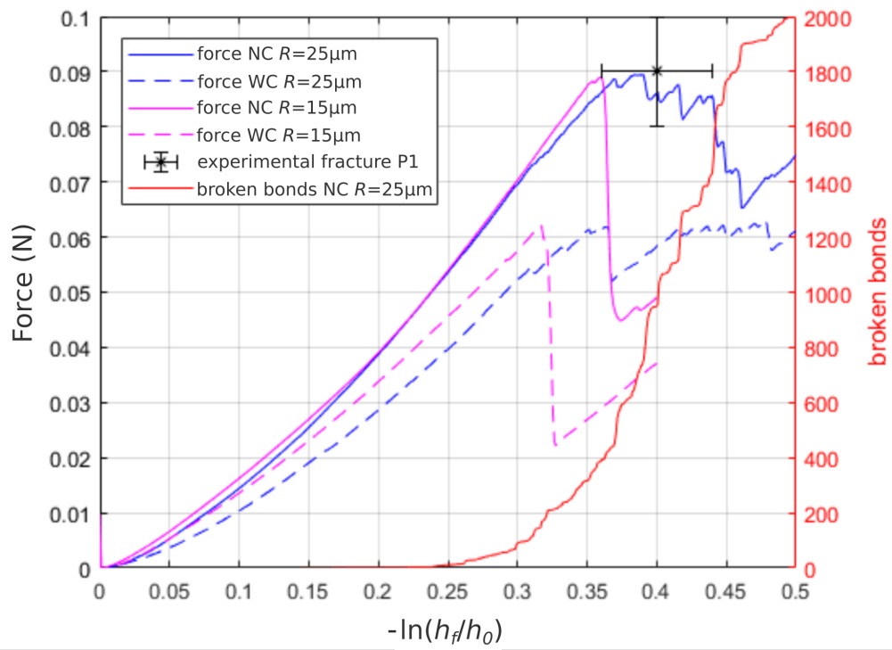
Figure 9: DEM compression of P1 with (WC) and without (NC) initial cracks generated from coarse ( 25\mu\text{m} ) and fine ( 15\mu\text{m} ) discrete elements. Experimental critical fracture of the particle is highlighted.
