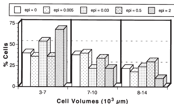
Fig. 3. Strombidium sulcatum . Distribution of cell volumes among ciliate populations after 3 d of incubation under different turbulence regimes ( \text{epi} = \epsilon , \text{cm}^2 \text{s}^{-3} ). Note that the ciliate populations from intermediate and high turbulence treatments contained a high portion of small cells
