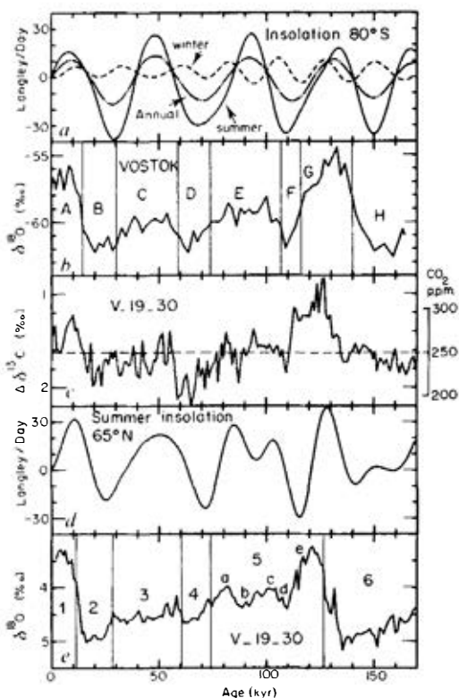
Fig. 4 Variation with time of: a , winter, summer and annual insulations at 80° S (ref. 59); b , \delta^{18}\text{O} in the Vostok ice (this work); c , \Delta\delta^{13}\text{C} in the V 19-30 deep-sea core 68 and indication of the \text{CO}_2 scale on the right; d , summer insolation at 65° N (ref. 59); e , \delta^{18}\text{O} in the V 19-30 deep-sea core 68 for Uvigerina Senticosa with an indication of the successive climatic stages.
