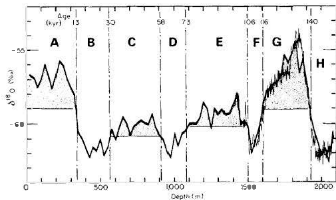
Fig. 1 ●xygen-18 versus depth in the Vostok ice with the definition of the successive stages and indication of the ages corresponding to the limits between these stages. The thick line is drawn from discontinuous data (one for each 25 m), the thin line corresponds to a continuous sampling between 1,400 and 2,083 m. For explanation of A-H, see text.
