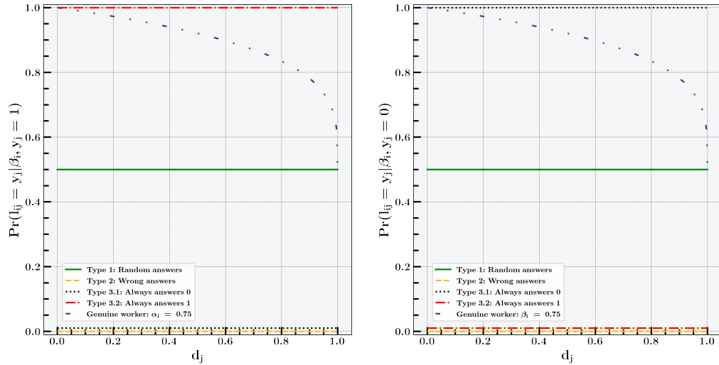
Fig. 5: Generating functions depicting the probability of correct answers for honest workers (with recall \alpha = 0.75 and specificity \beta = 0.75 ) and Type 1, Type 2, and Type 3 spammers.
