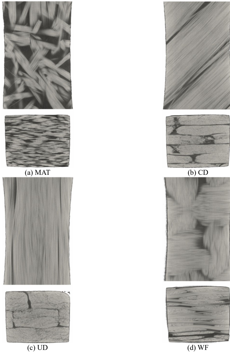
Fig. 3 Front and top mid-slices of the scanned FRPs with four different fiber architectures
