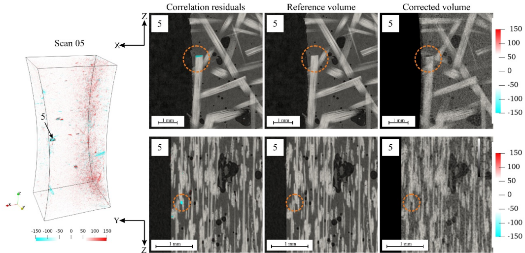
Fig.10 Correlation residuals (scan 05) of characteristic subregion 5 laid over the corresponding mesostructure sections (first column). The second column corresponds to the reconstructed data in the reference configuration f , while the third column displays the deformed volume corrected by the measured displacement field. The dashed orange circles indicate the area of elevated correlation residuals in two perpendicular planes.
