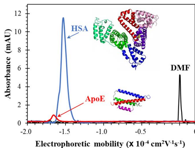
Figure 2. Electropherograms of HSA and ApoE ( 1.44 \mu\text{M} ) in a capillary pre-conditioned with 30 mM ACB (pH 7.4). The separation was performed with E=14 \text{ kV} , and the signals obtained with a UV-Vis detector ( \lambda = 200 \text{ nm} ).
