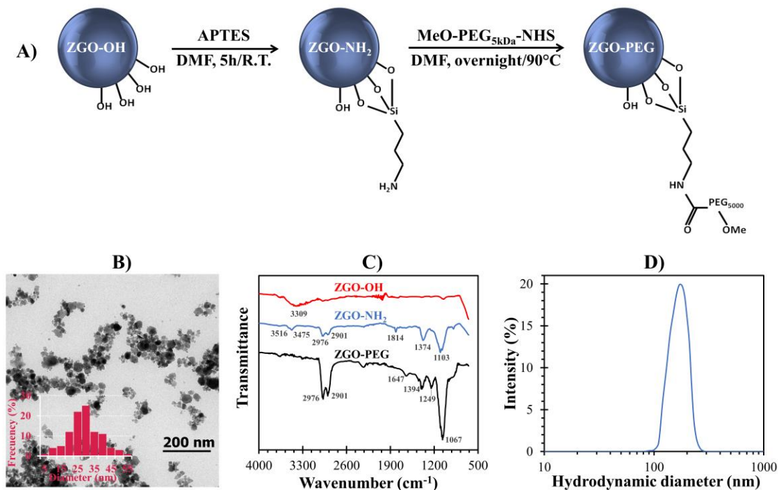
Figure 1. A) Schematic representation of the \text{ZnGa}_{1.995}\text{Cr}_{0.005}\text{O}_4 surface functionalization sequence, B) TEM image of the ZGO-PEG NPs. The inset shows the corresponding histogram for size distribution. C) FTIR-ATR spectra of the intermediary functionalized ZGO-NPs. D) DLS profile of ZGO-PEG in pH 7.4 ACB 30 mM.
