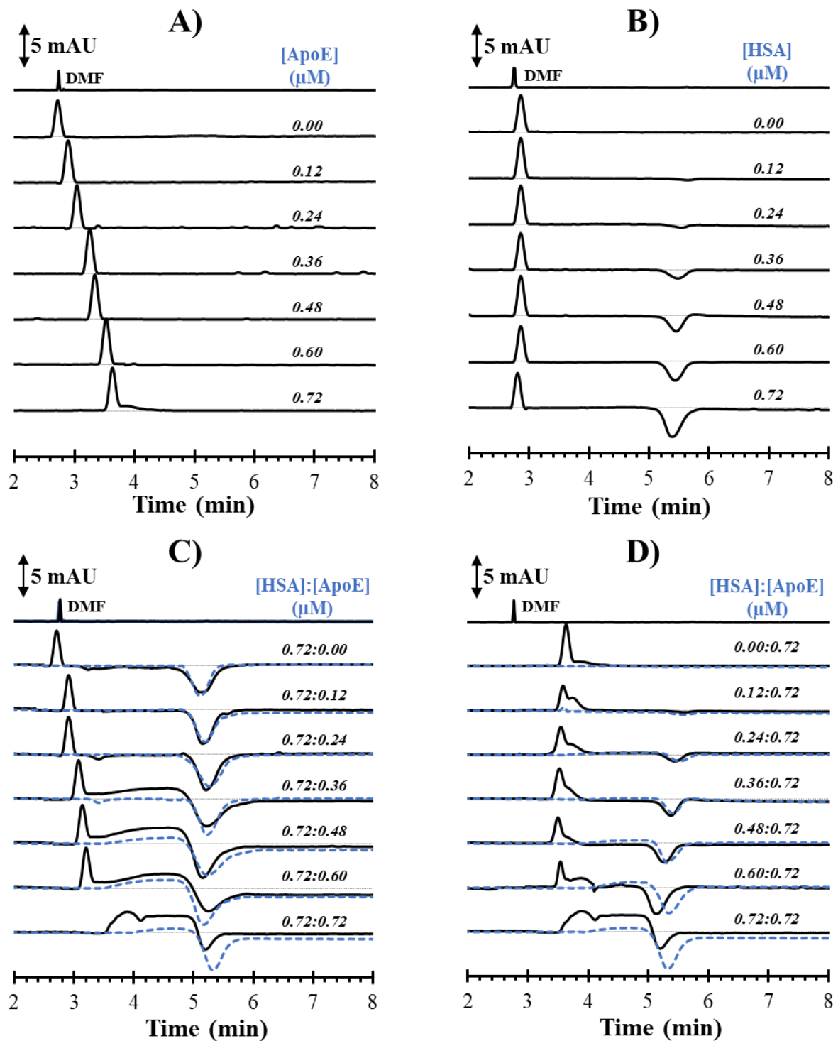
Figure 4. Electropherograms for evaluation of the cooperative interactions between ZGO-PEG and binary systems of proteins. a) interactions between ZGO-PEG and ApoE. b) interactions between ZGO-PEG and HSA. interactions between ZGO-PEG and a mixture of proteins at different ratios: c) HSA concentration was fixed and ApoE varied, and d) ApoE concentration was fixed and HSA varied. In all the systems, the continuous lines correspond to the electropherograms obtained upon the ZGO-PEG injection, while the superimposed dashed lines in c) and d) correspond to the ACB injection. The indicated values are the final protein concentrations in the mixtures. The analyses were performed in 15 mM ACB (pH 7.4). E=14.0 kV.
