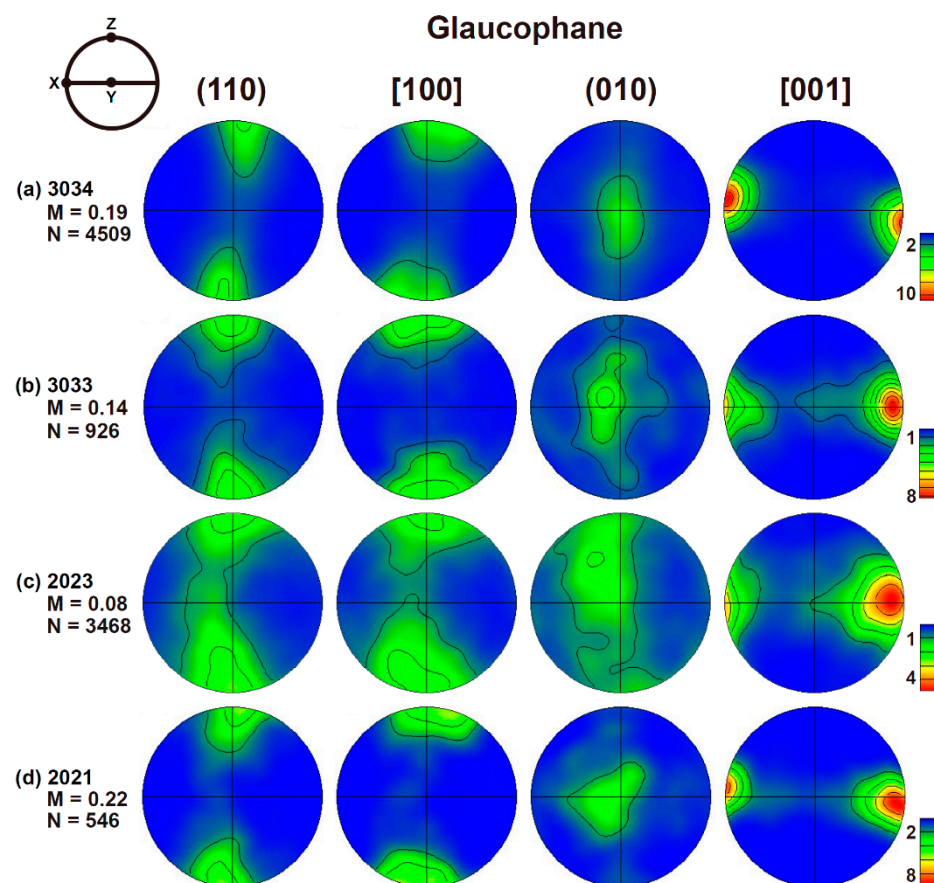
Figure 6. (a–d) Pole figures of glaucophane. The x and z directions correspond to the lineation and direction normal to the foliation, respectively. A 20^\circ half-scan width and a 5^\circ cluster size are used. Contours represent the CPO strength, and multiples of uniform distribution (m.u.d.) are shown as color bars. The higher the number of the bar, the higher is the CPO strength. M: misorientation index; N: number of grains.
