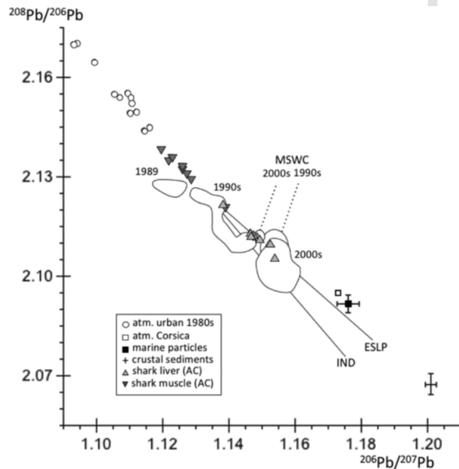
Fig. 3. Comparison of Pb imprints ( ^{208}\text{Pb}/^{206}\text{Pb} vs. ^{206}\text{Pb}/^{207}\text{Pb} ) in Centroscymnus coelestis muscle and liver of AC sharks to those of marine particles and atmospheric deposition (MP and Atm in Fig. 1). Atmospheric Pb isotope ratios of French urban areas (Bollhofer and Rosman, 2001; Carignan et al., 2005; Cloquet et al., 2006; Elbaz-Poulichet et al., 1984, 1986; Monna et al., 1995, 1997; Roy, 1996; Veron et al., 1999; Widory, 2006; Widory et al., 2004) are shown for three decades (1980s, 1990s, 2000s) along with mean non-contaminated sediment imprints of the open Western Mediterranean Sea (Ferrand et al., 1999; Angelidis et al., 2011).
