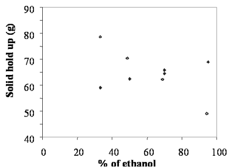
Figure 8. Moving mass (◇) and dead mass (◆) as a function of the percentage of ethanol ( \dot{m}_{SI} = 11.33 \text{ g min}^{-1} ).
