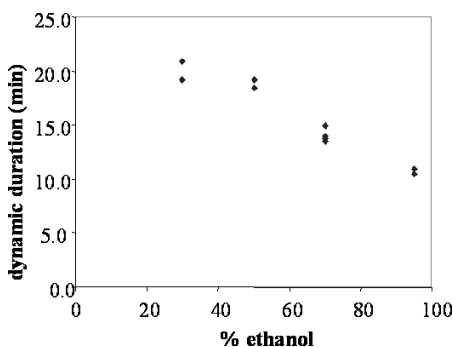
Figure 6. Dynamic duration time as a function of the ethanol concentration ( \dot{m}_{SI} = 11.33 \text{ g min}^{-1} ).
