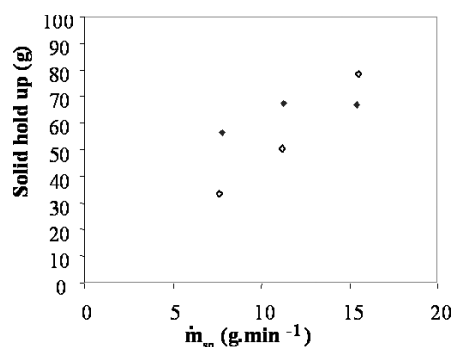
Figure 7. Moving mass ( \diamond ) and dead mass ( \blacklozenge ) as a function of the solid mass flow rate (95 % ethanol).
