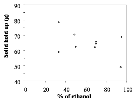
Figure 8. Moving mass ( \diamond ) and dead mass ( \blacklozenge ) as a function of the percentage of ethanol ( \dot{m}_{ST} = 11.33 g min -1 ).
