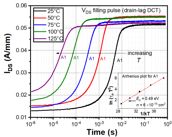
Figure 5. The drain current transient (DCT) spectroscopy of AlGaN/GaN HEMT acquired with the drain-lag filling pulse ( V_{DS} pulsed from 10 to 20 V for 100 ms during the trap-filling phase) at increasing temperature levels. The Arrhenius plot for A1 is displayed in the inset.
