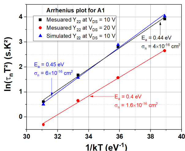
Figure 13. Arrhenius plots for the trap A1 obtained from the measured Y_{22} parameters at V_{DS} = 10 \text{ V} and 20 \text{ V} are shown along with the simulation case at V_{DS} = 10 \text{ V} .
