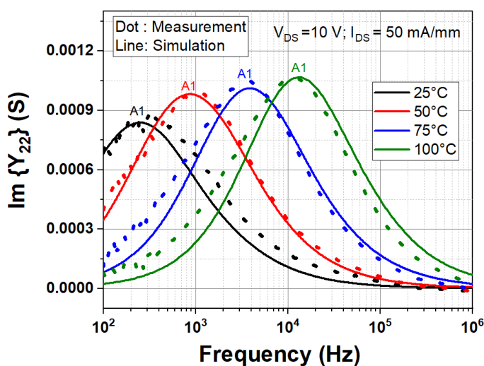
Figure 14. The simulated LF Y_{22} characteristics at V_{DS} = 10 \text{ V} are validated with the measured spectra for different temperatures of 25 to 100 \text{ }^\circ\text{C} .
