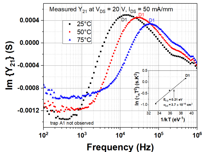
Figure 17. The measured LF Y_{21} parameters obtained at V_{DS} = 20 V, I_{DS} = 50 mA/mm for various temperatures (25 to 75 °C) show only the surface donor at E_C = -0.21 eV. The buffer trap A1 is not detected for this bias condition.
