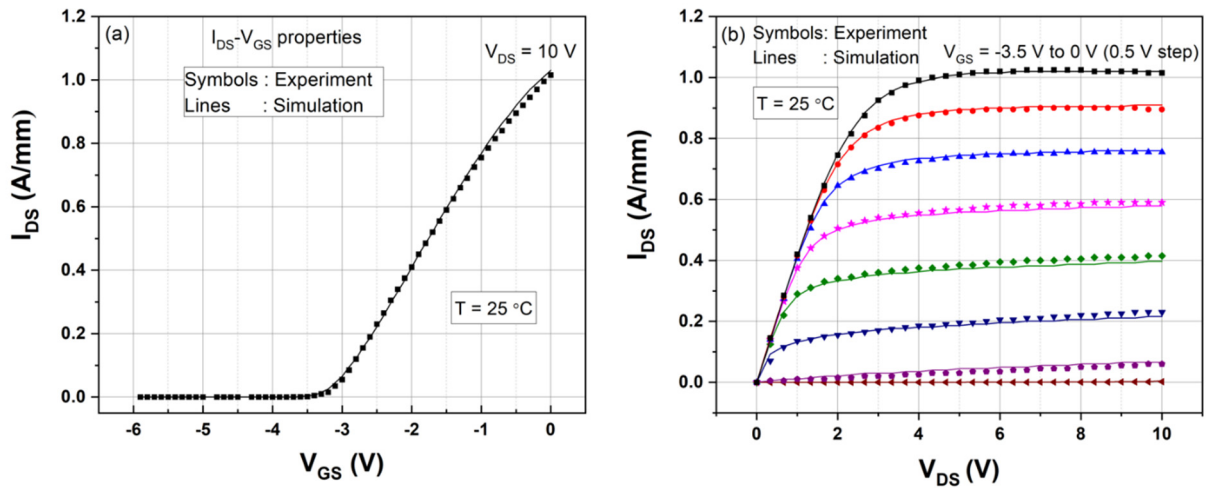
Figure 11. Simulated (a) transfer ( I_{DS} - V_{GS} ) and (b) output ( I_{DS} - V_{DS} ) properties of the Fe-doped AlGaIn/GaN HEMT are validated with the measured DC results.
