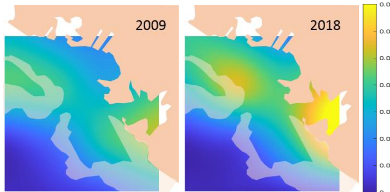
Fig 3. Turbidity from remote sensing
