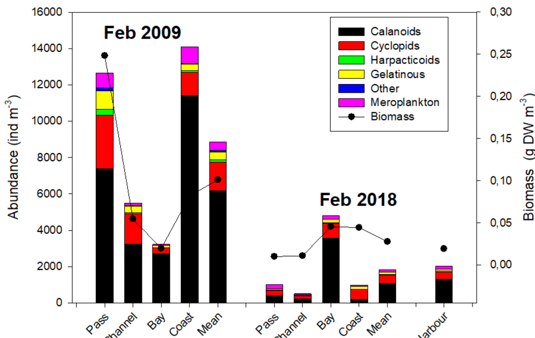
Fig 4. Zooplankton abundance and biomass. (Harbour not sampled in 2009).
