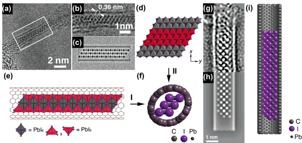
Figure 4. (a and b) conventional HRTEM image and detail (from boxed region) showing a \text{PbI}_2 1D crystal formed within a 1.6 nm diameter SWNT. (c) Scherzer focus HRTEM image simulation based on the structure model in e. (d) Single layer of \text{PbI}_2 showing the ‘origin’ of the 1D fragment, indicated in red. (e) Composite model and (f) space-filling end-on view showing \text{PbI}_2 fragment inside a (12,12) SWNT. The latter shows how this tubule could distort in order to accommodate the derived asymmetric \text{PbI}_2 crystal fragment. The arrow I indicates the \text{PbI}_2 fragment projection in parts a–e. (g) Reconstructed phase image of a \text{PbI}_2 fragment formed in a 1.6 nm diameter SWNT. (h) Matching multislice simulation. (i) Composite model used to calculate the simulation in h. The projection of this fragment is indicated by arrow II in f.
