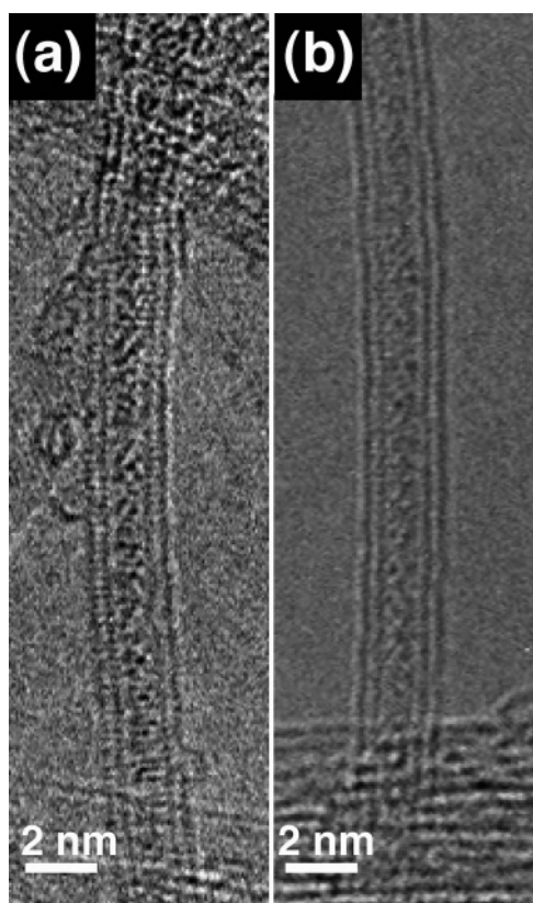
Figure 6. (a and b) Two examples of HRTEM images obtained near to Scherzer defocus of narrow DWNTs filled with noncrystallizing \text{PbI}_2 .
