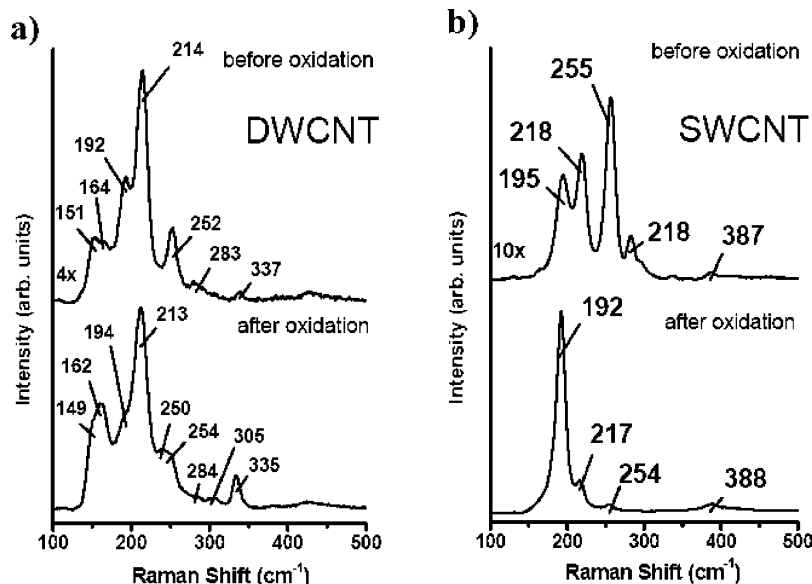
Figure 2. RBM frequency range of the Raman spectra of (a) DWCNTs and (b) SWCNTs before and after nonisothermal oxidation. The RBMs of the DWCNTs show no significant changes after oxidation, suggesting that oxidation of the nanotubes did not occur. The RBMs of the SWCNT sample show structural changes within the sample, starting with the oxidation of smaller tubes and the disappearance of higher RBM frequencies. Spectra were acquired at room temperature using a 633 nm laser excitation.
