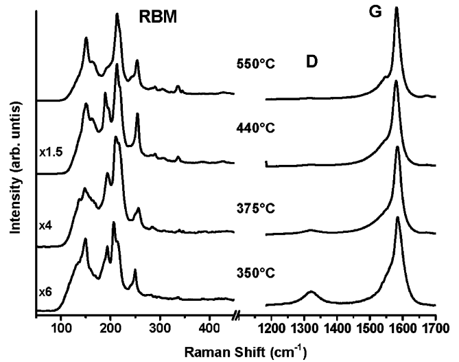
Figure 7. First-order Raman spectra of DWCNT after isothermal oxidation at different temperatures recorded at room temperature using a 633 nm laser excitation. The R value shows no changes for oxidation temperatures below 350 °C. At higher temperatures, R reaches a minimum after a certain time, depending on the temperature, until it becomes zero at 550 °C (D band disappears).
