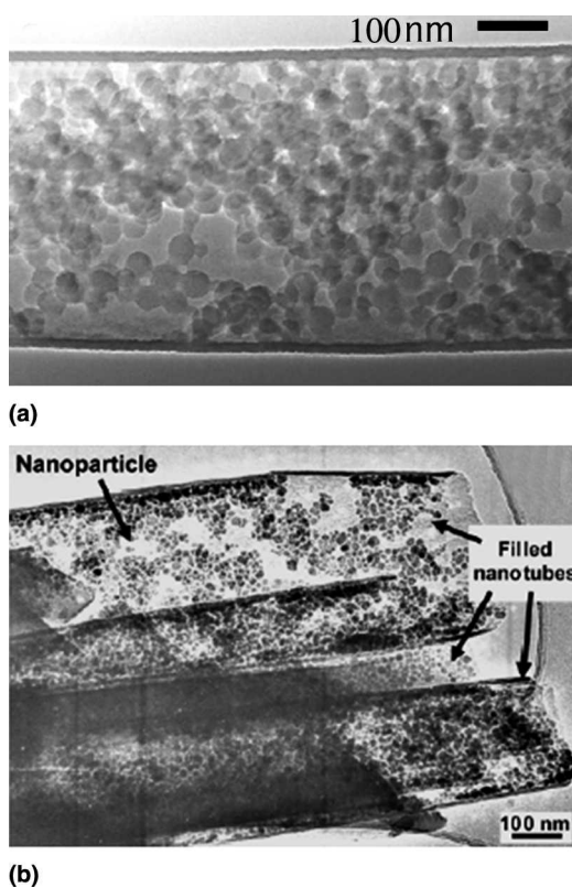
FIG. 5. Examples of MWNTs filled with nanoparticles via the suspension method (liquid route), taken from pioneering works. (a) Polystyrene nanobeads initially suspended in ethylene glycol. 53 (b) Fe 3 O 4 nanoparticles initially suspended in water- or organic-based “ferrofluids.” 54 Reprinted with permission of American Chemical Society.
